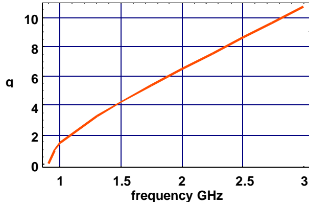
Figure 3. The values of q for the TE_{z_{11}} mode as a function of frequency for an Azimuthally Propagating, Truncated, Cylindrical, Coaxial Waveguide defined by the parameters: r_1 = 5in = 0.127 m , r_2 = 6in = 0.1524 m and a = 6.5 inches.
