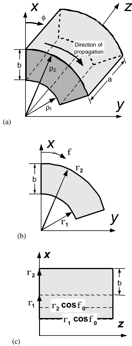
Figure 2. The geometry of the azimuthally propagating, truncated, cylindrical coaxial waveguide: (a) 3-D perspective drawing; (b) plane view of the xy -plane; and (c) plane view of the xz -plane.
