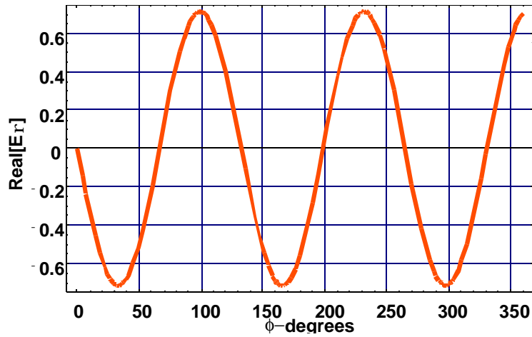
Figure 6. The value of the E_r component of the electric field of the TEz_{11} mode as a function of azimuthal position.
