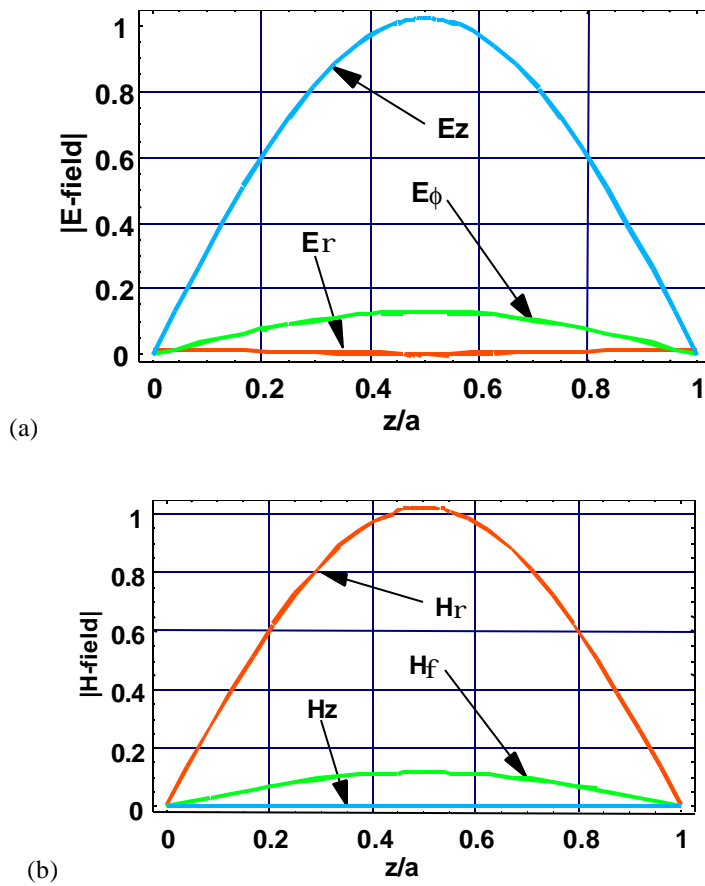
Figure 8. The electromagnetic field distribution of the various field components for the TMz_{11} mode: (a) normalized electric field; and (b) normalized magnetic field.
