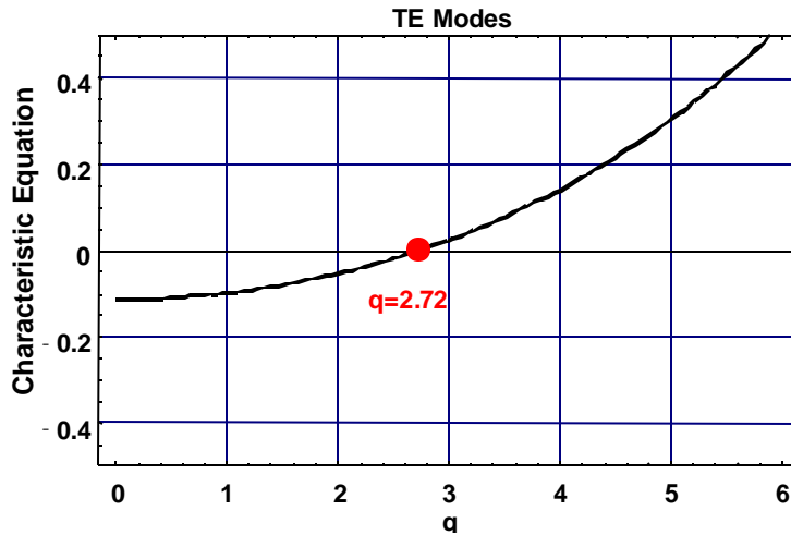
Figure 4. The characteristic equation of the TE z11 mode for an Azimuthally Propagating, Truncated, Cylindrical, Coaxial Waveguide defined by the parameters: r_1 = 5\text{ in} = 0.127\text{ m} , r_2 = 6\text{ in} = 0.1524\text{ m} and a = 6.5\text{ inches} .
