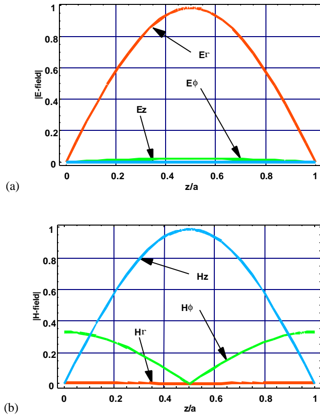
Figure 5. The electromagnetic field distribution of the various field components in an Azimuthally Propagating, Truncated, Cylindrical, Coaxial Waveguide defined by the parameters: r_1 = 5\text{ in} = 0.127\text{ m} , r_2 = 6\text{ in} = 0.1524\text{ m} and a = 6.5 inches for the TE z 11 mode: (a) normalized electric field; and (b) normalized magnetic field.
