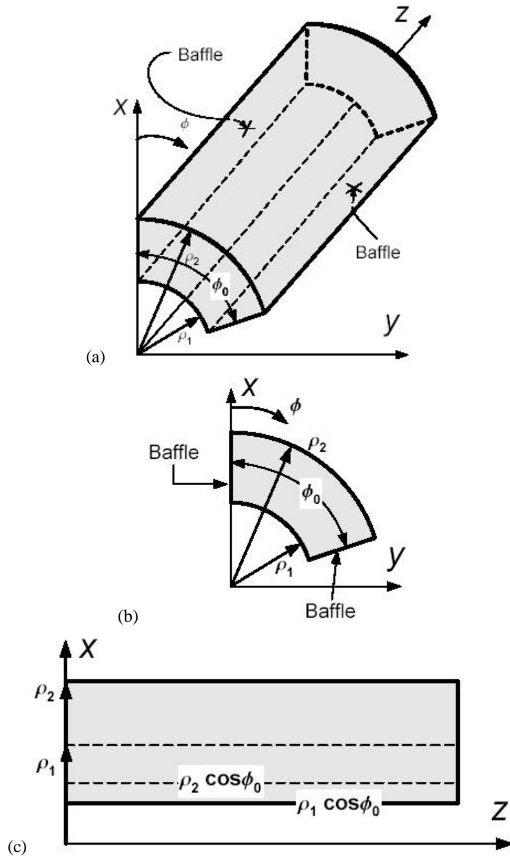
Figure 1. The geometry of the double baffled cylindrical coaxial waveguide: (a) 3-D perspective drawing; (b) plane view of the xy-plane; and (c) plane view of the xz-plane.
