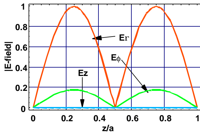
Figure 7. The electric field distribution of the various field components in an Azimuthally Propagating, Truncated, Cylindrical, Coaxial Waveguide defined by the parameters: r_1 = 5in = 0.127\ m , r_2 = 6in = 0.1524\ m and a = 6.5 inches for the TEz_{21} mode.
