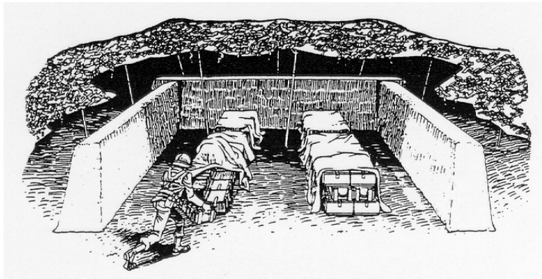
Figure 40. Soil Cement Revetment.
