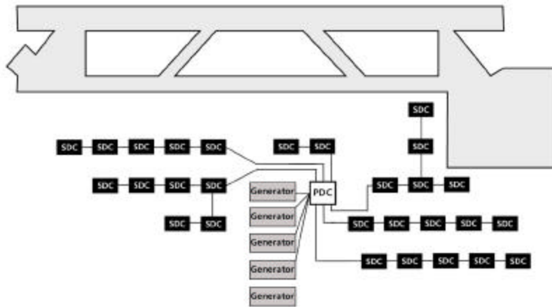
Figure 23. Radial Electrical Distribution System For 1,100-Person Power Plant(s).
