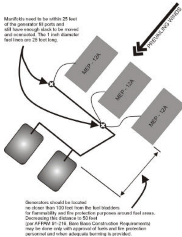
Figure A2.1. Basic Generator and Fuel System Layout.
