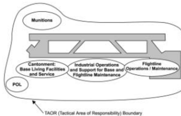
Figure 22. Linear Base Layout.
