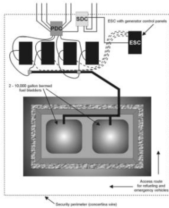
Figure A2.3. Power Plant General Layout.
