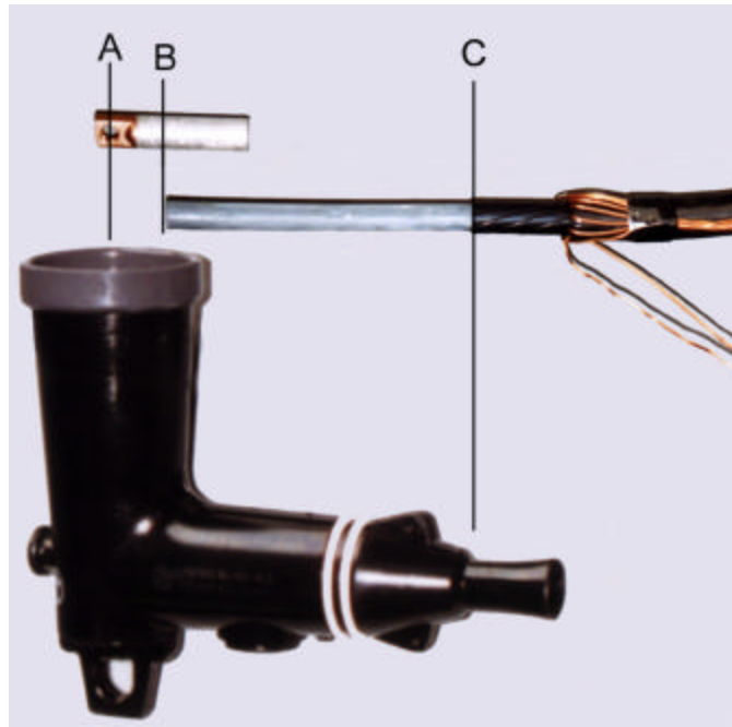
Figure A4.7. Guide for Determining Shield Removal.
