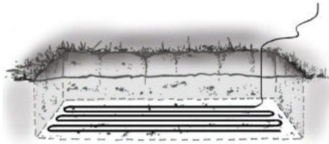
Figure 43. Typical Equipment Laced Wire Grounding Installation.
