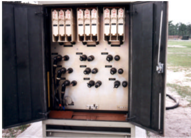
Figure 52. Connect Cables to SDC Input Bushings.
