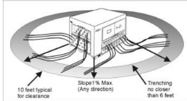
Figure 37. Typical PDC Clearances.
