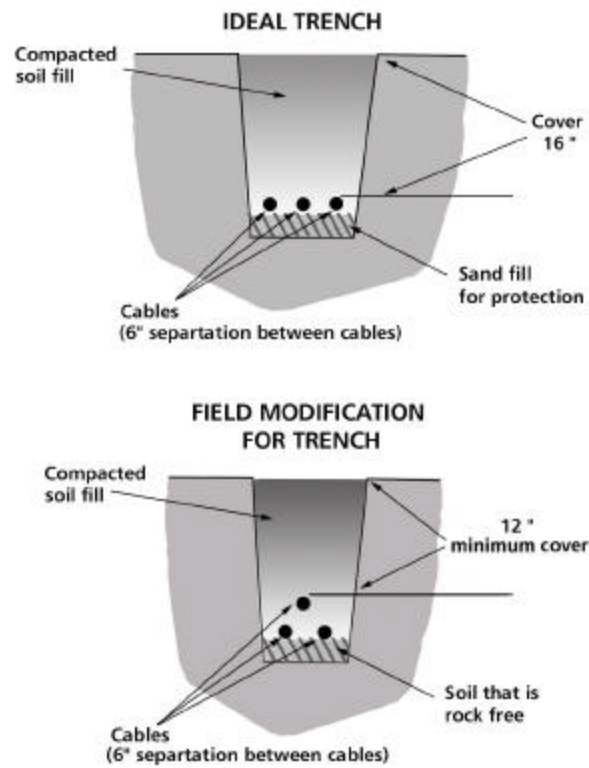
Figure 46. Trench and Cable Detail.
