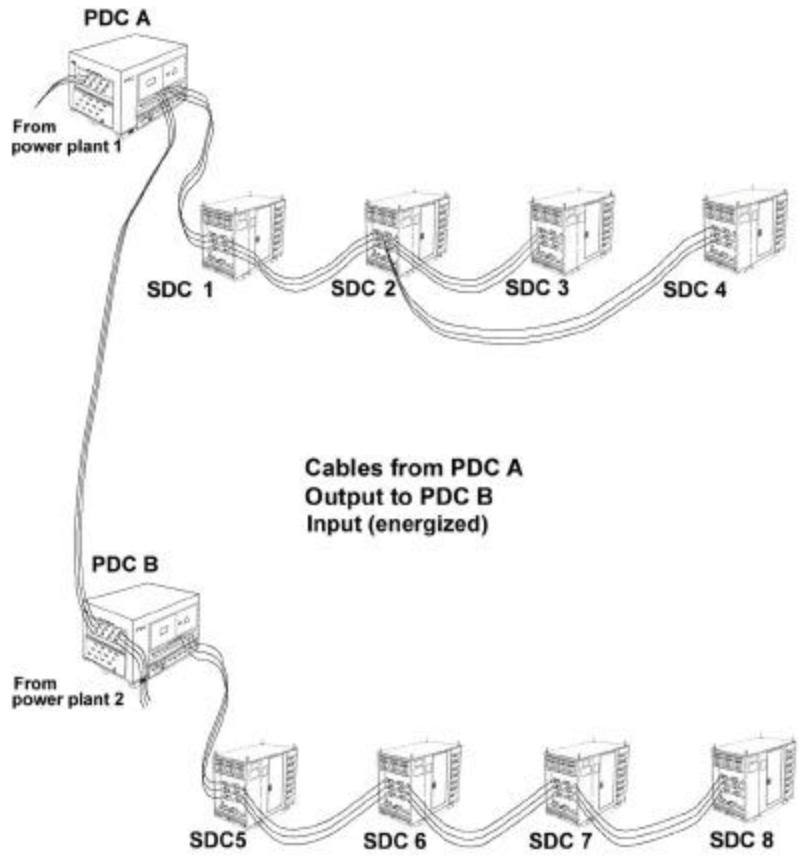
Figure 33. Typical Connection between Two PDCs.
