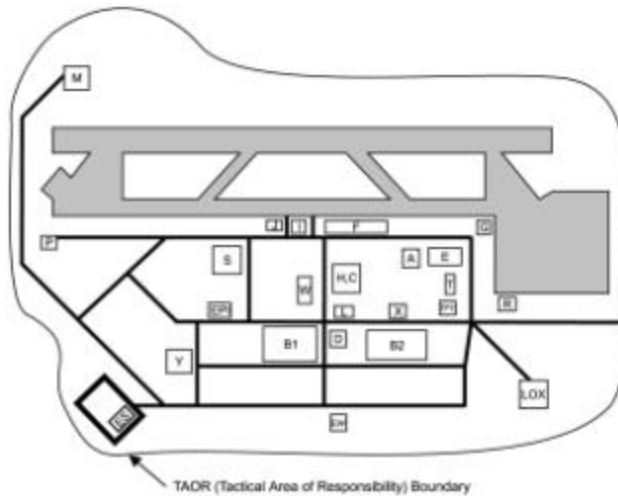
Figure 29. Typical 1,100-Person Layout with Major Roadway Grid.
