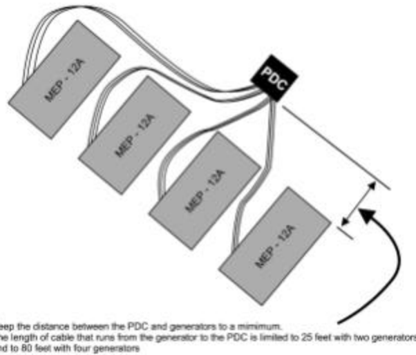
Figure 38. Placement of PDC near Generators.
