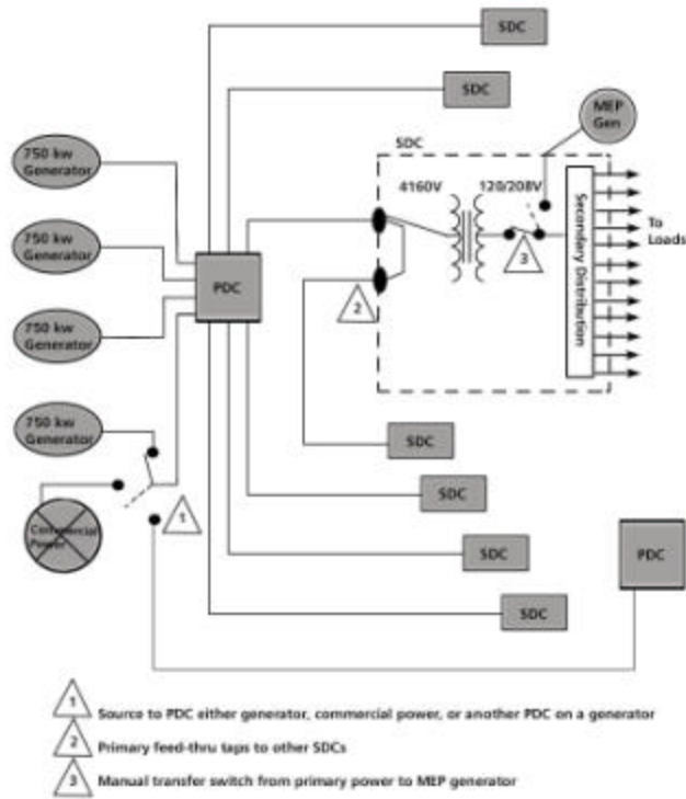
Figure 16. Basic Electrical Distribution System Schematic.
