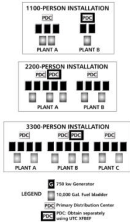
Figure 27. Typical Plant Layout Groupings.
