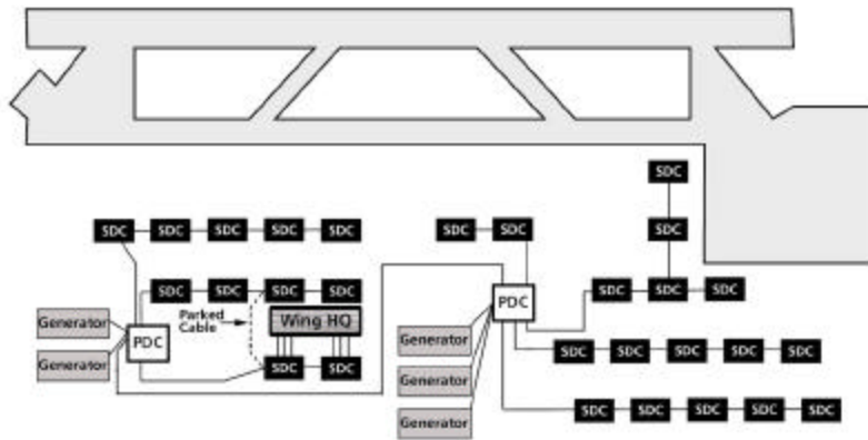
Figure 26. Critical Facility SDCs Connected By Parked Cables.
