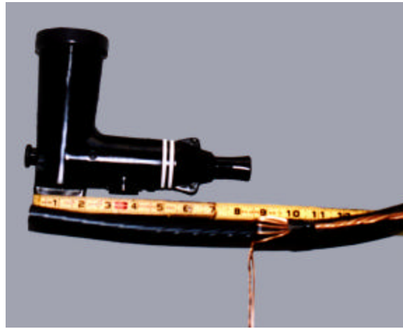
Figure A4.6. Cut the Cable for the Distance of the Load Break Elbow from the Bent Wires.
