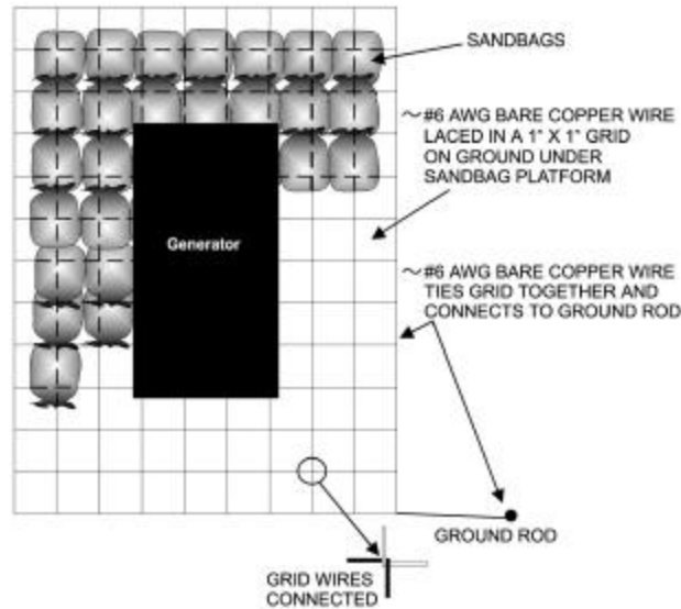
Figure 44. Typical Equipment Grounding Grid Platform Installation.
