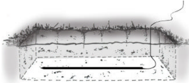
Figure 42. Typical Equipment Horizontal Ground Rod Installation.
