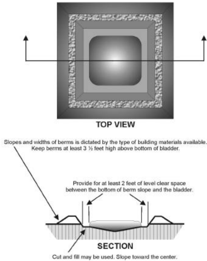
Figure A2.2. Bladder and Berm Detail.
