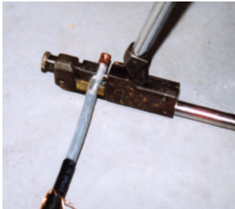
Figure A4.9. Crimp the Contact Bushing's Barrel.
