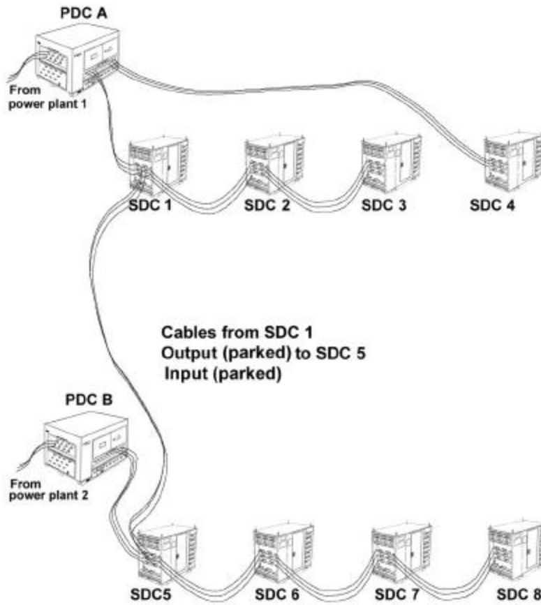
Figure 34. Typical Parked Cables between Two SDCs on Different Circuits.
