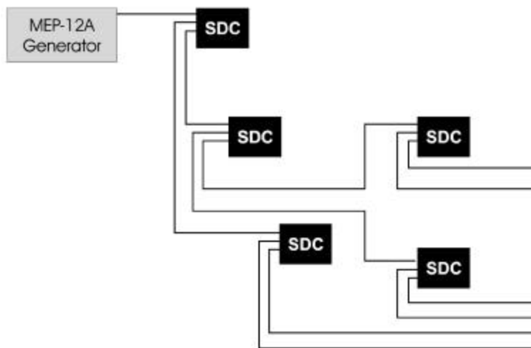
Figure 63. Branch Connected SDCs with a MEP-12A Generator.
