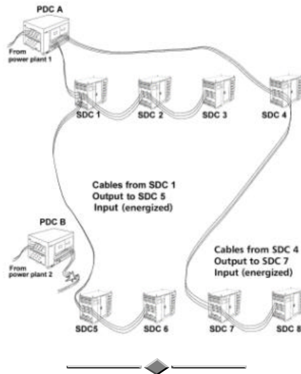
Figure 35. Rerouting of Cables to Prevent Overloading of Remaining PDC.
