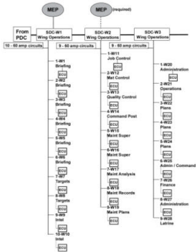
Figure 32. Example SDC Circuit for Wing Operations Group.
