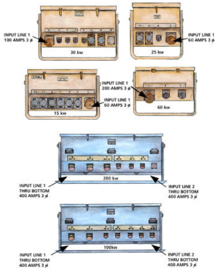
Figure 12. Typical Power Distribution Panels.
