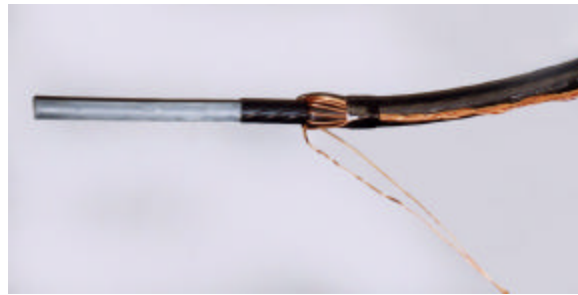
Figure A4.3. Remove Shield from the Insulation.
