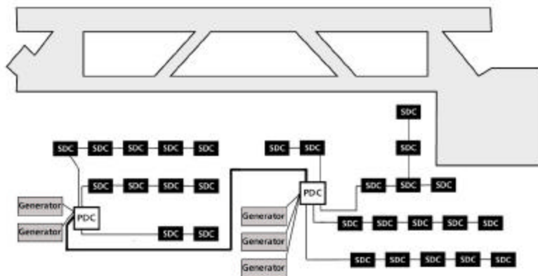
Figure 25. Interconnected Electrical Distribution System for 1,100-Person Power Plant(s).
