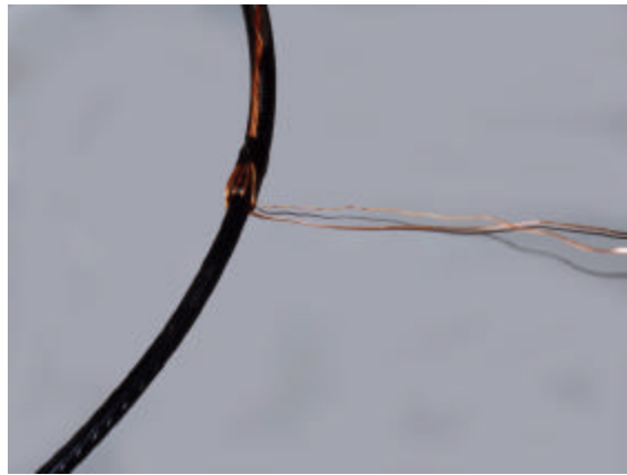
Figure A4.2. Concentric Neutral Wires with Temporary Wrapping.
