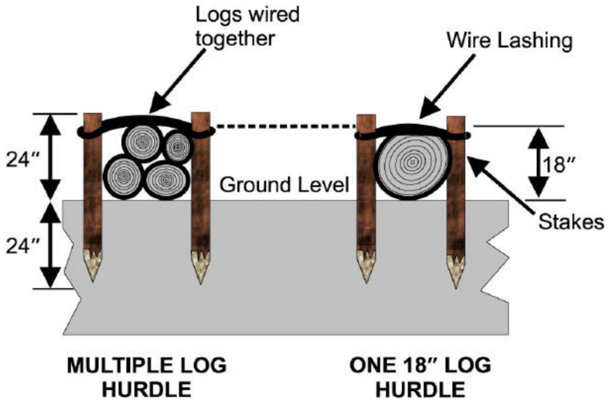
Figure 49. Log Hurdles.
