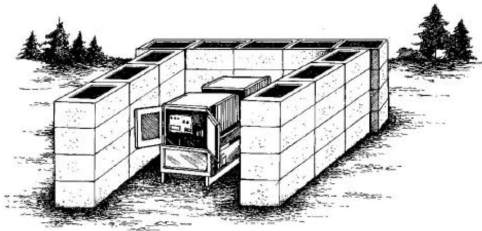
Figure 31. Concrete Chamber Soil Bin.
