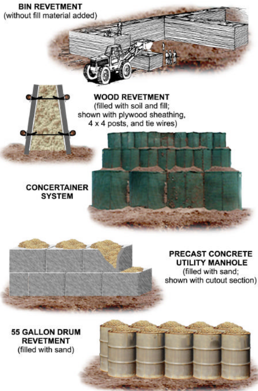
Figure 3. Containment Concepts.
