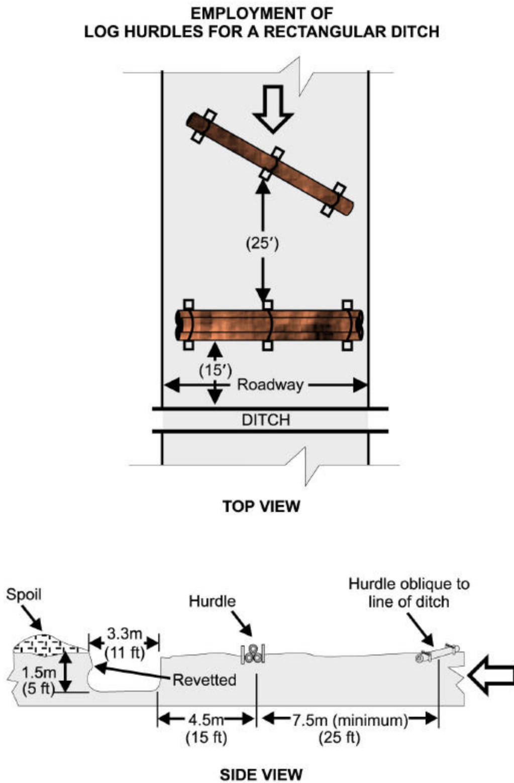
Figure 47. Locating Log Hurdles.
