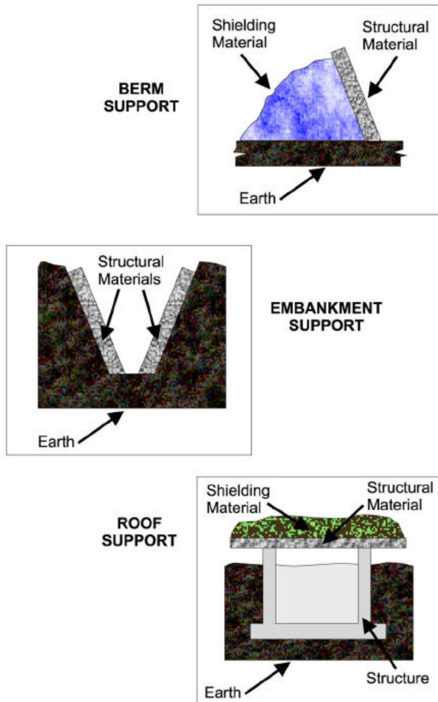
Figure 2. Bracing Concepts.
