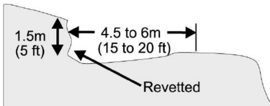
SIDEHILL CUT DITCH
