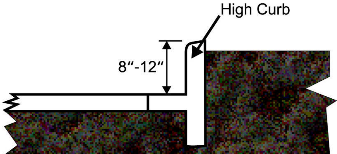
Figure 64. Straight Faced Curb.
