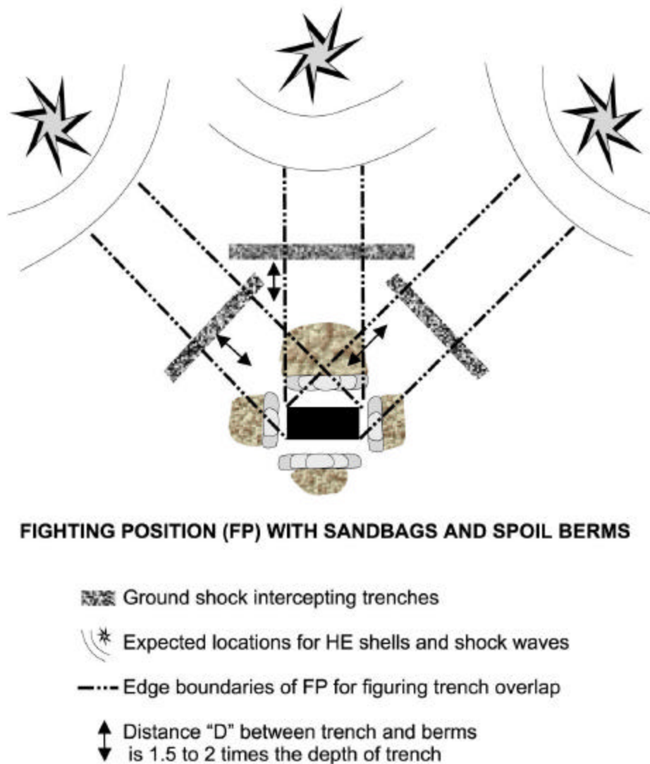
Figure 77. Placement of Ground Shock Intercepting Trenches.
