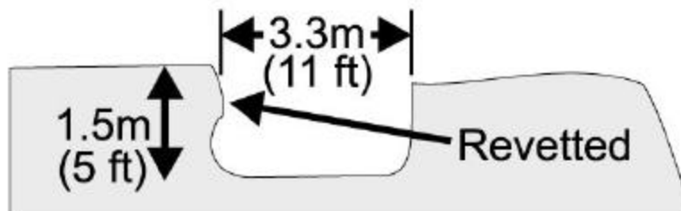
RECTANGULAR DITCH
