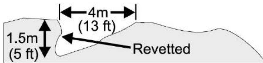
TRIANGULAR DITCH
