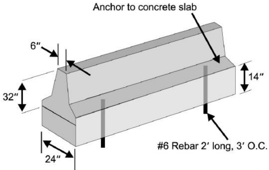
Figure 67. Jersey Barrier.
