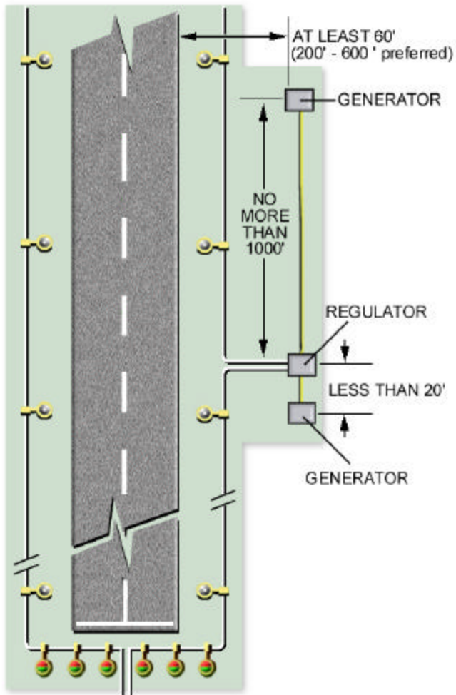
Figure 10. Generator and Regulator Placement.
