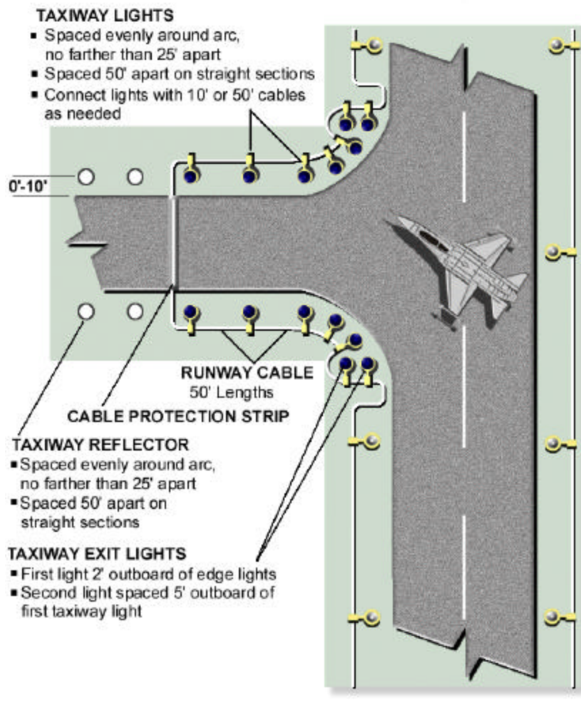
Figure 9. Taxiway Light Placement.
