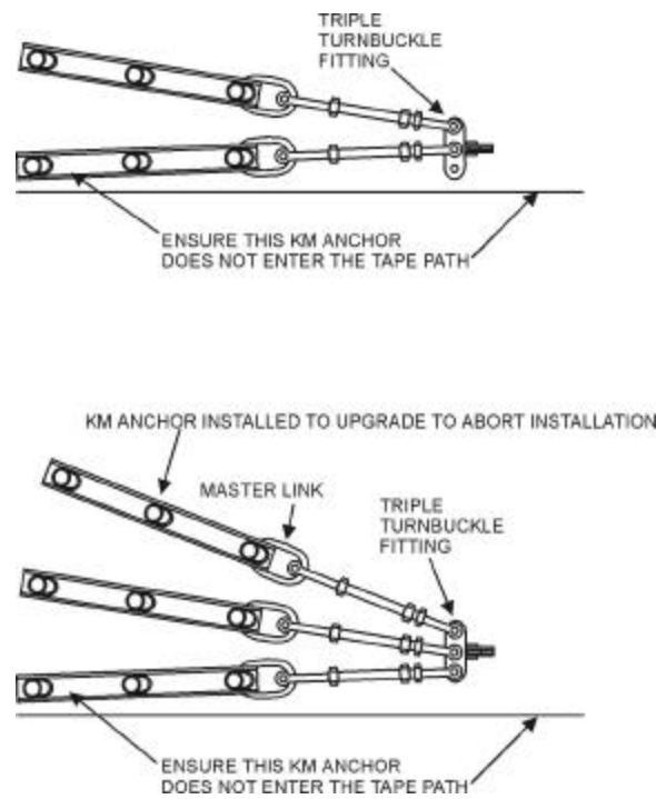
Figure 79. Triple-Turnbuckle Fitting Upgraded from Two to Three KM Stake Lines.
