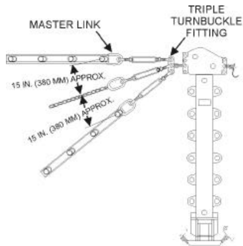
Figure 121. Locating the Second Stake Line.
