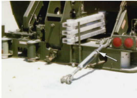
Figure 34. Locknut End Always Toward the Anchored Equipment.
