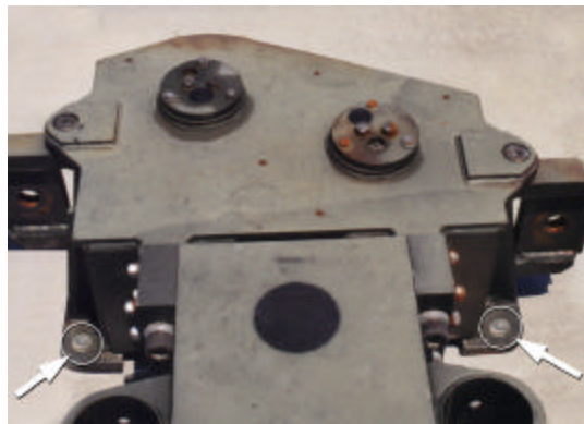
Figure 129. Install Two Concrete Anchor Bolts at Front of LWFB.
