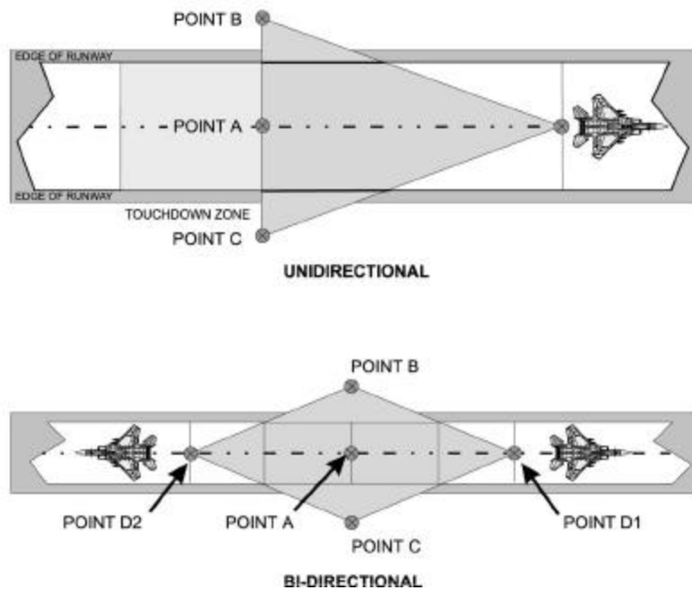
Figure 19. Tape Sweep Areas to Be Cleared.
