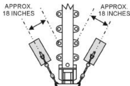
Figure 128. Align Back Anchor Plates on Concrete.
