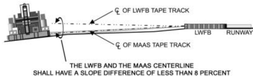
Figure 18. Angle of Decline Between MAAS and the Fairlead Beam.
