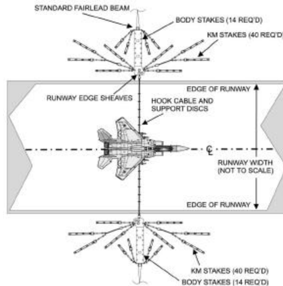
Figure 119. Standard Fairlead Beam on Soil with KM Stake Lines – Bi-directional Operation.
