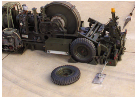
Figure 47. Store Tire Away from Runway – Both MAAS Trailers.
