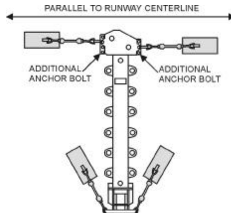
Figure 126. Typical LWFB Anchoring Requirements on Concrete.
