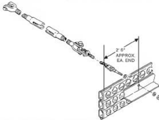
Figure 132. Typical Fabrication of Chain and Deadman.
