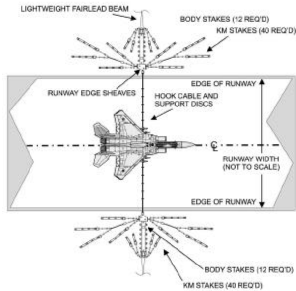
Figure 118. LWFB on Soil – Bi-directional Operation.
