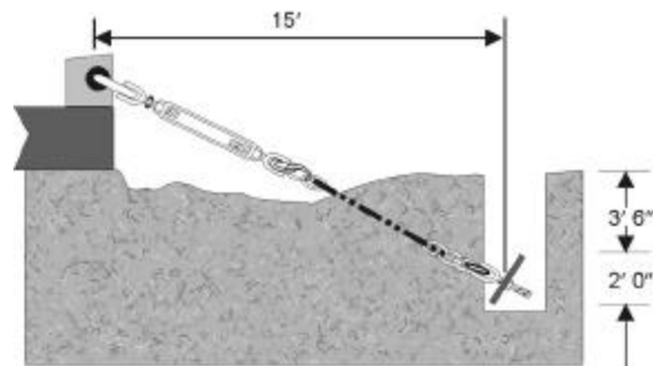
Figure 134. Typical Deadman, Chain, and Trench Layout – Elevation View
