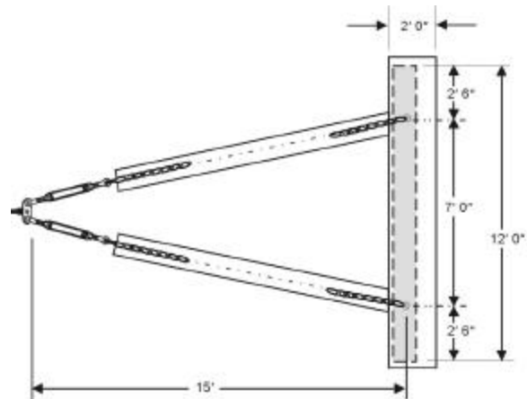
Figure 134. Typical Deadman, Chain, and Trench Layout – Elevation View
