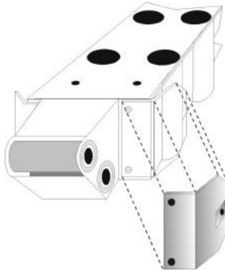
Figure 120. Standard Fairlead Beam Adapter Brackets (Right Side Detail)
