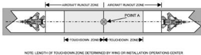
Figure 6. Establishing Centerline Point A – Bi-directional Operations.
