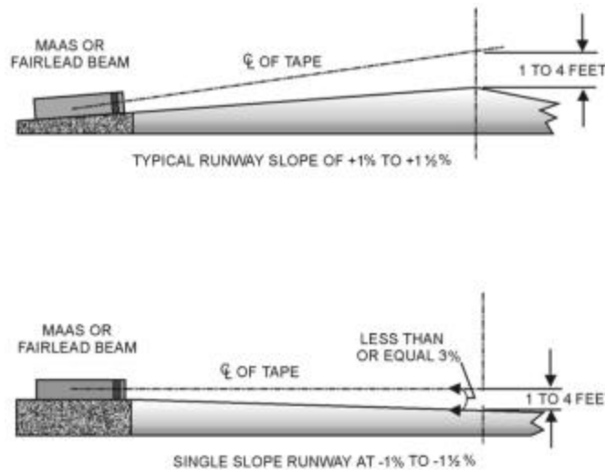
Figure 17. Projection of Tape Centerline Above Runway.
