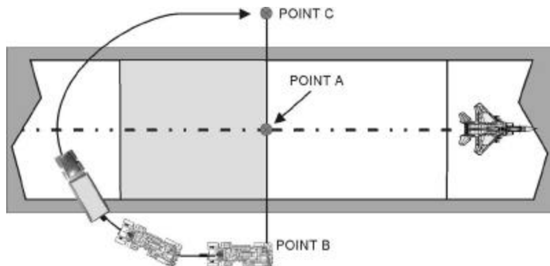
Figure 20. Positioning the MAAS Trailers.
