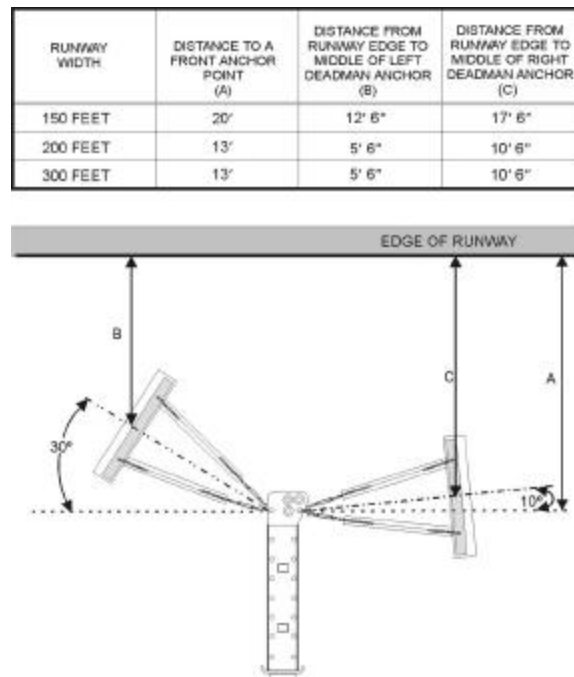
Figure 131. Typical Standard Fairlead Beam Layout.
