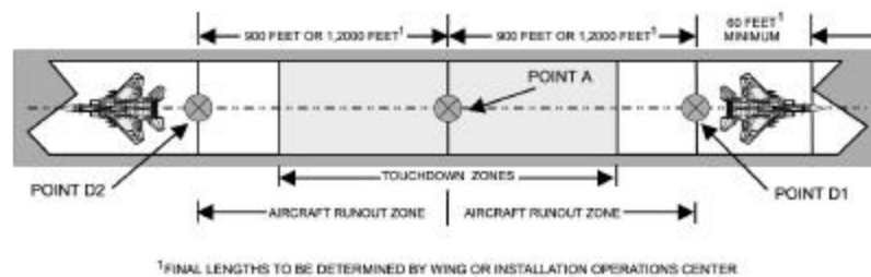
Figure 8. Establishing Centerline Points D1 and D2 – Bi-directional Operation.
