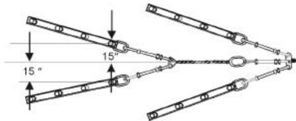
Figure 117. Locating the Rear Stake Lines.
