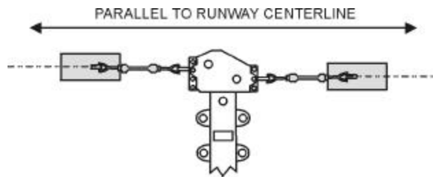
Figure 127. Align Front Anchor Plates on Concrete.
