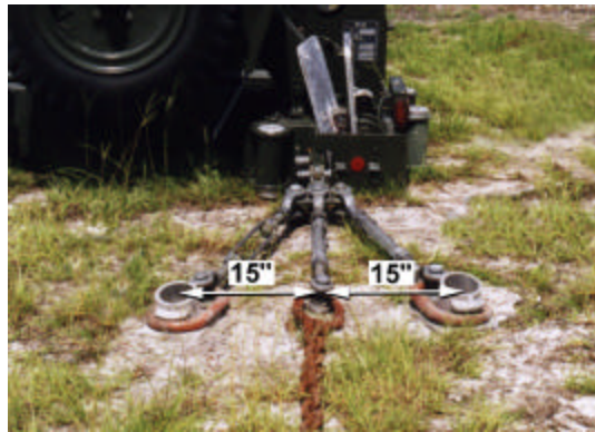
Figure 116. Locating the Front Stake Lines.
