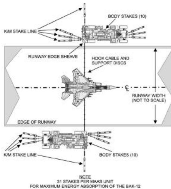
Figure 81. MAAS on Soil for Heavyweight, Bi-directional Operation.
