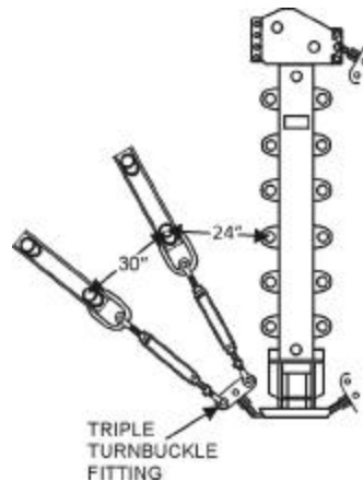
Figure 123. Locating the Rear Stake Lines.
