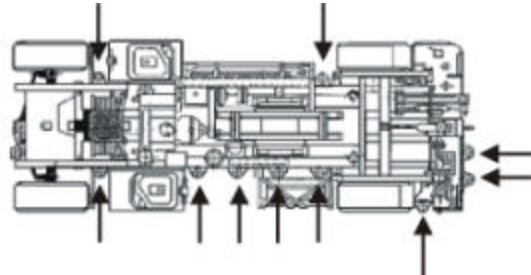
Figure 111. Stake Body Locations on the MAAS.
