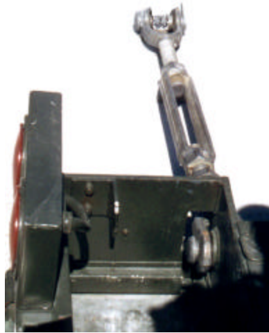
Figure 49. Right Rear Anchor Point with Turnbuckle – Both MAAS Trailers.
