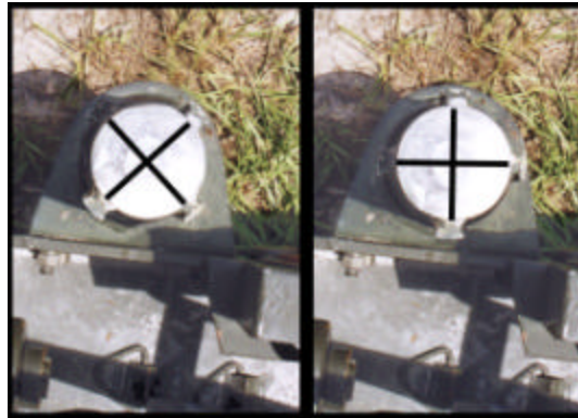
Figure 113. Proper Stake Orientation with the Body.
