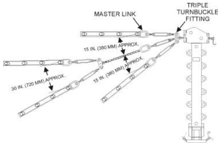
Figure 122. Locating the Front Rear Stake Lines.
