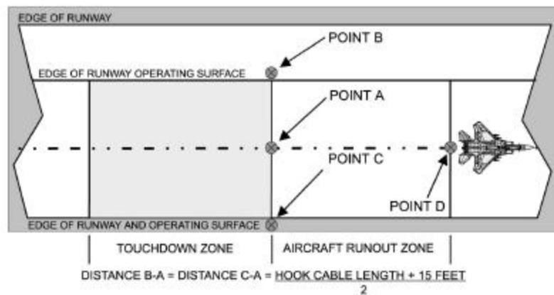
Figure 9. Establishing MAAS Set Points B and C.
