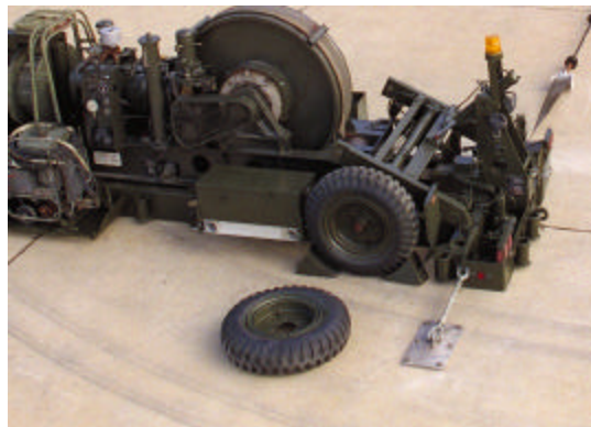
Figure 39. Store Tire Away from Runway – Right MAAS Trailer.
