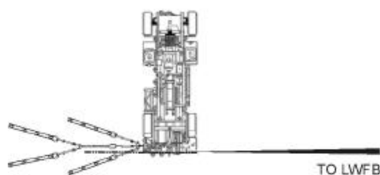
Figure 110. Detailed Layout of 26-Stake System.
