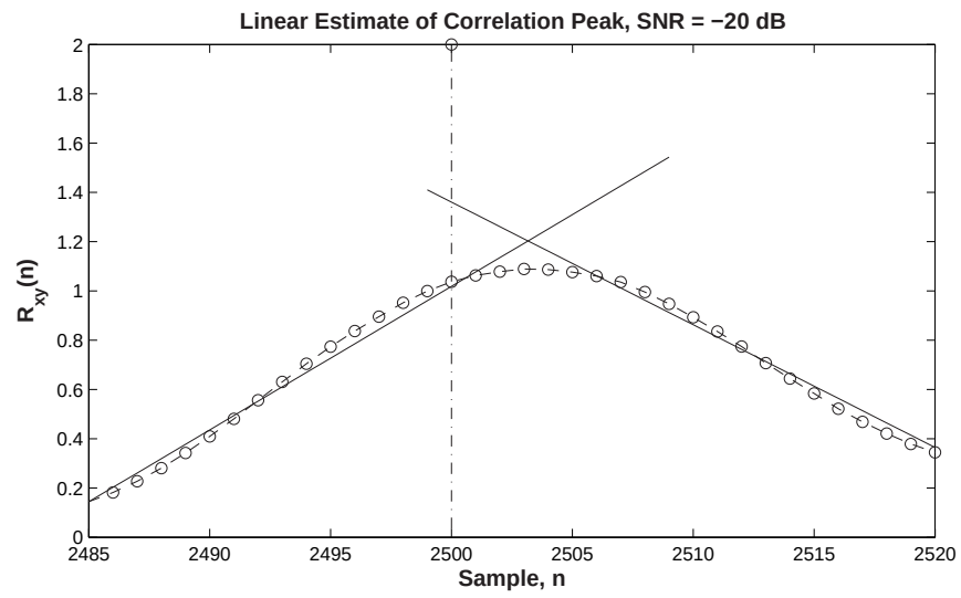
Figure 2.11: Linear Fit Peak Estimator
