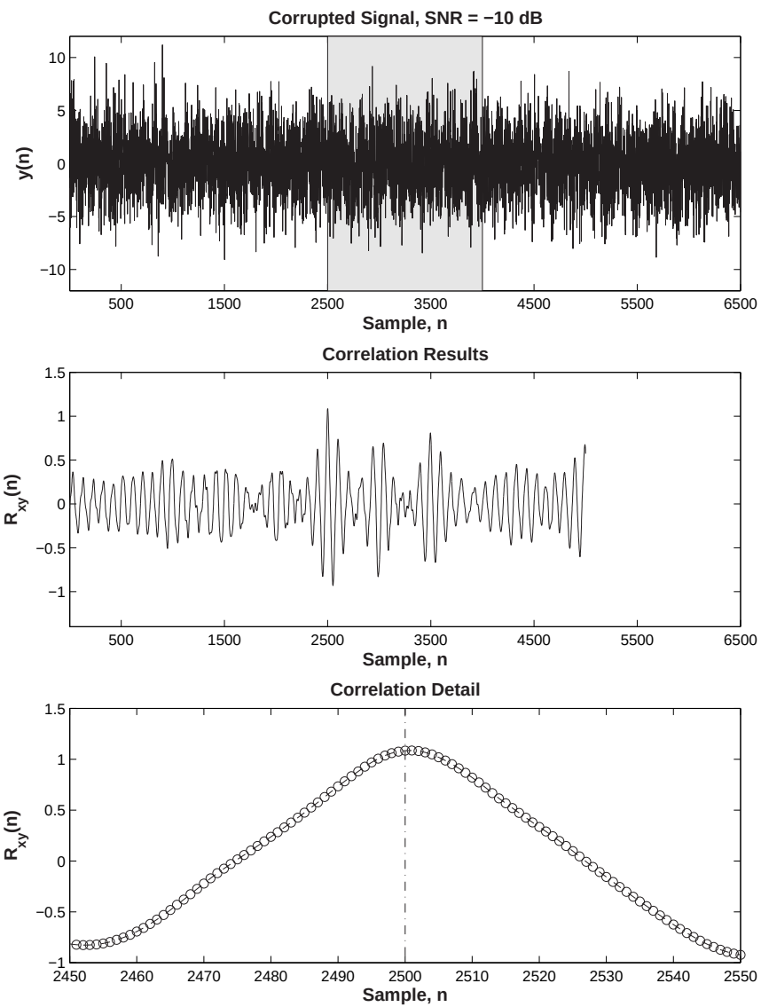
Figure 2.9: Correlation Results, SNR = -10 dB (Compensated to Indicate the Start of the Desired Signal)
