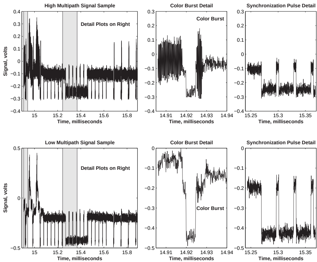
Figure 4.8: Low and High Multipath Signal Samples from Data Set 3
