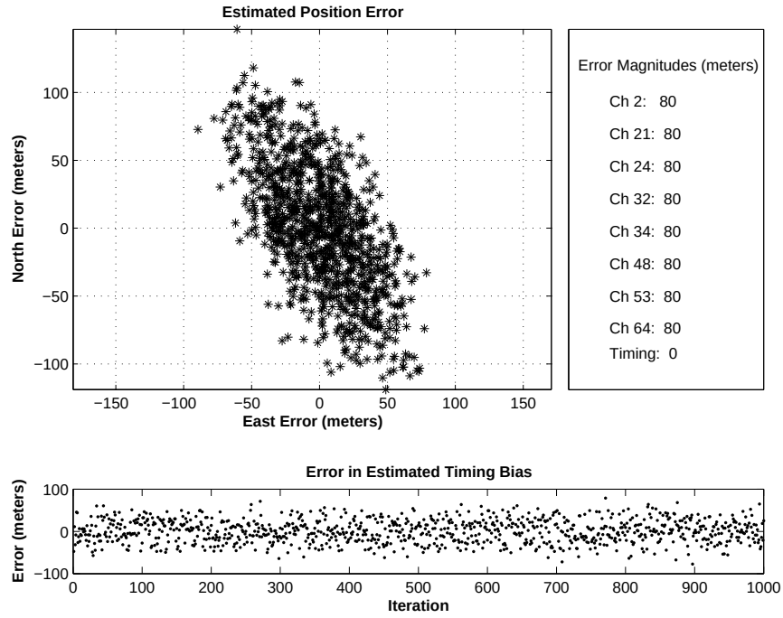
Figure 4.13: Simulated Position Estimation Error, High Multipath Errors and 0 Meter Timing Bias
