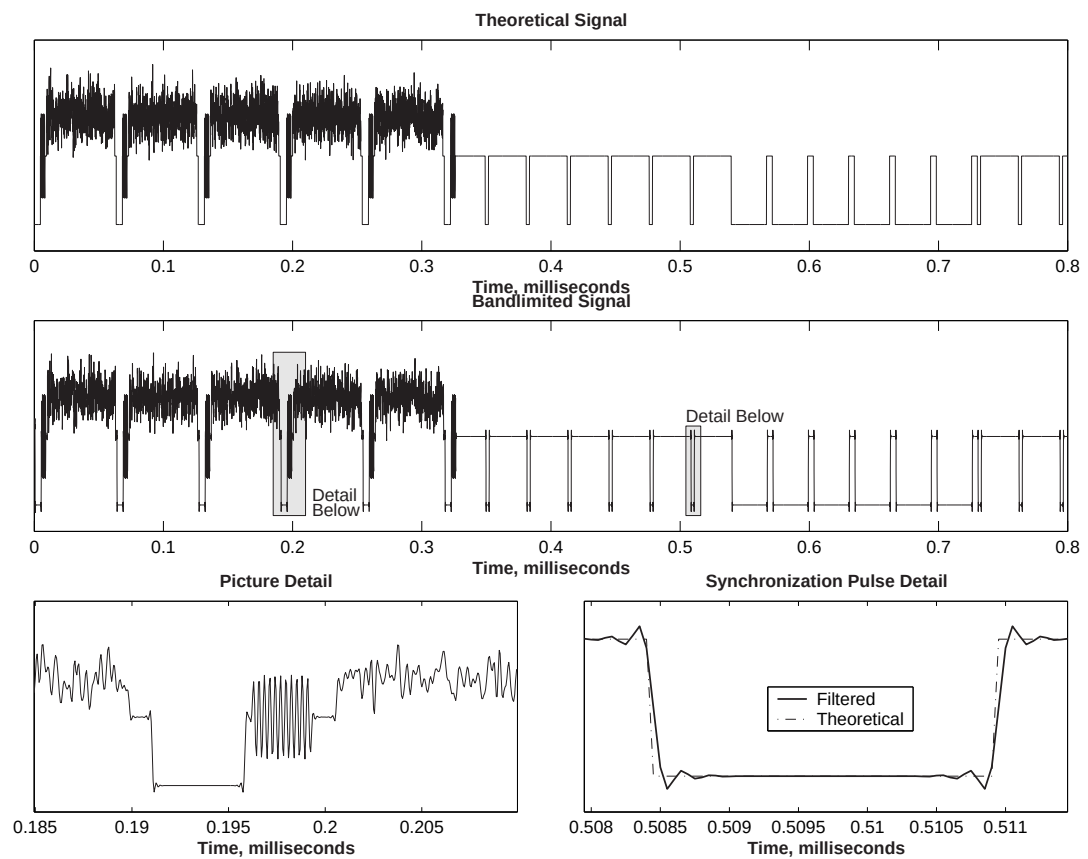
Figure 3.5: Effects of FIR Filter Bandlimiting the Video Signal
