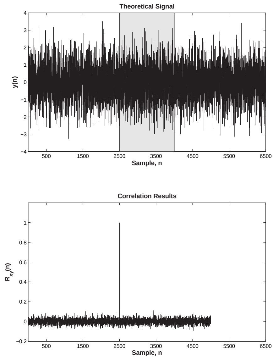
Figure 2.12: Correlation Results, Random Signals (Compensated to Indicate the Start of the Desired Signal)
