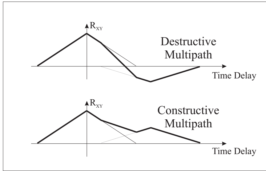
Figure 2.14: Multipath Effects on the Correlation Peak
