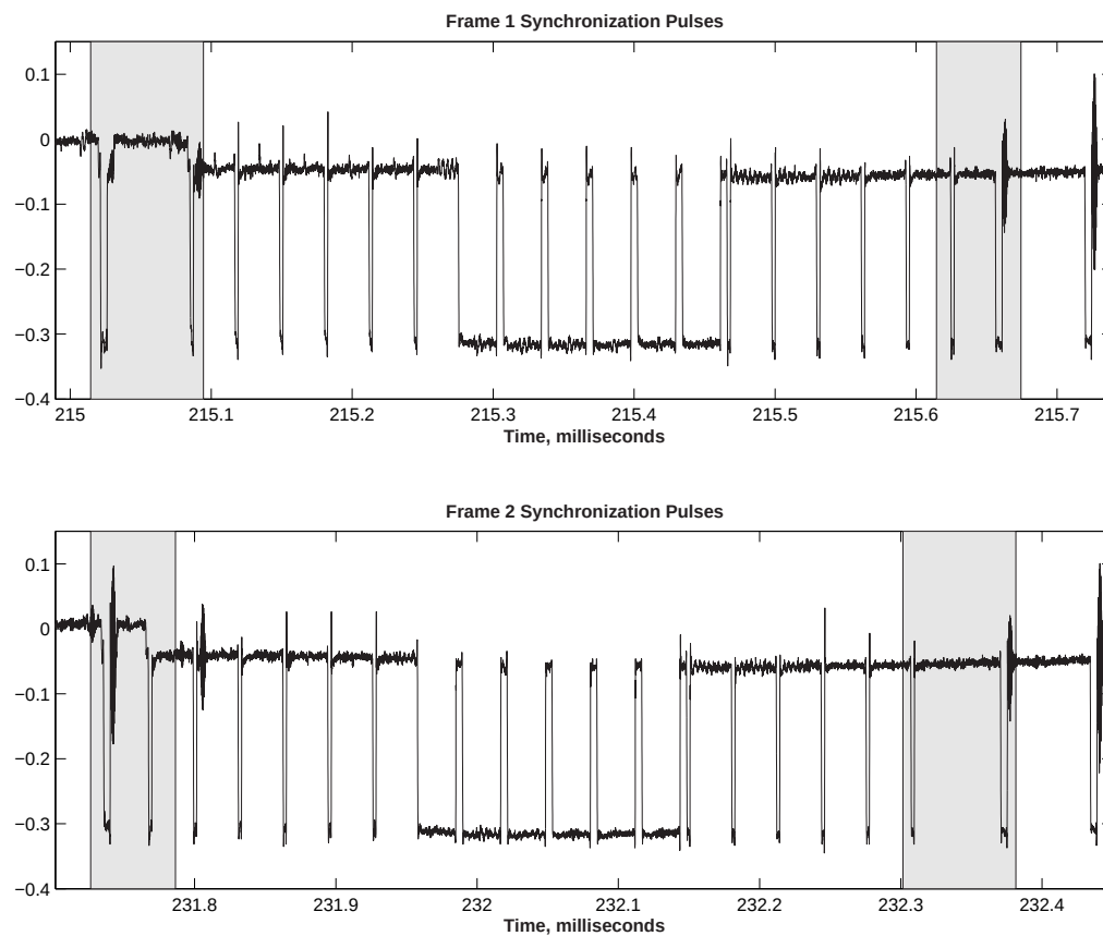
Figure 3.7: Comparison Between Sampled Frame 1 and Frame 2 Synchronization Pulses—VCR Video Encoder
