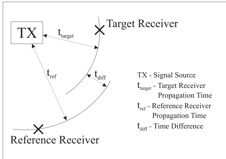
Figure 2.1: Illustration of TDOA Range Estimates
