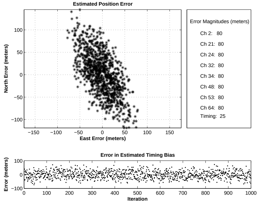
Figure 4.14: Simulated Position Estimation Error, High Multipath Errors and 25 Meter Timing Bias
