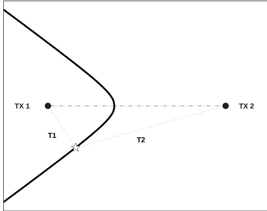
Figure 1.3: Locus of Possible Positions from Single Time-Difference Measurement in a Hyperbolic Navigation System
