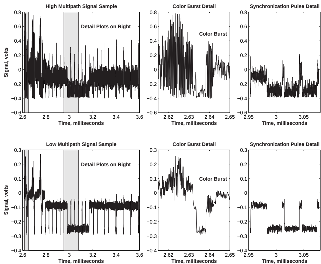
Figure 4.7: Low and High Multipath Signal Samples from Data Set 2
