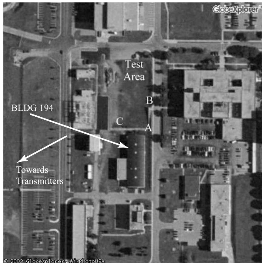
Figure 3.15: High Multipath Environment
