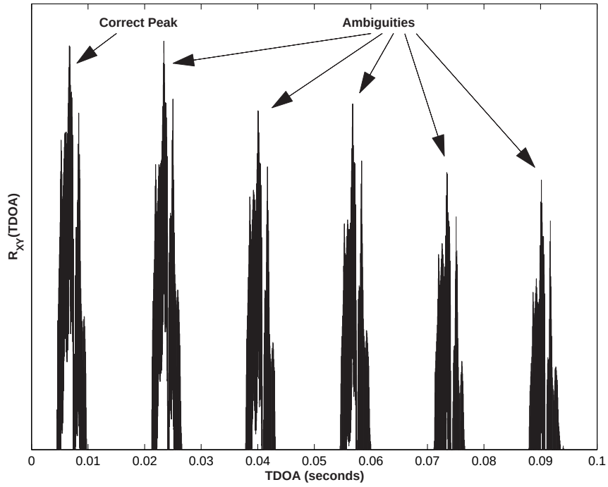
Figure 3.13: Potential Ambiguities From Successive Synchronization Pulses
