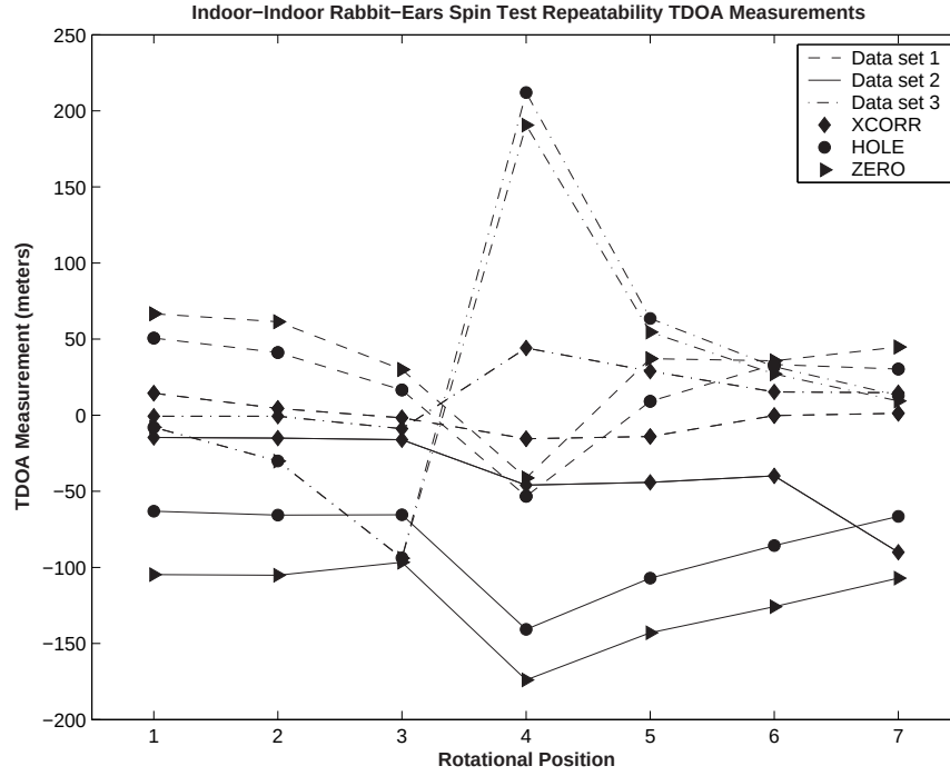
Figure 4.4: Indoor-Indoor Rabbit Ears Spin Test Repeatability TDOA Measurements (meters)—True TDOA: 0 meters
