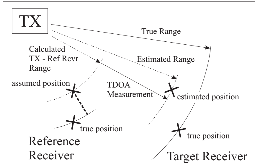
Figure 1.2: Reference Receiver Errors
