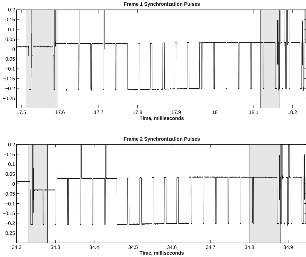
Figure 3.6: Comparison Between Sampled Frame 1 and Frame 2 Synchronization Pulses—DVD Video Encoder
