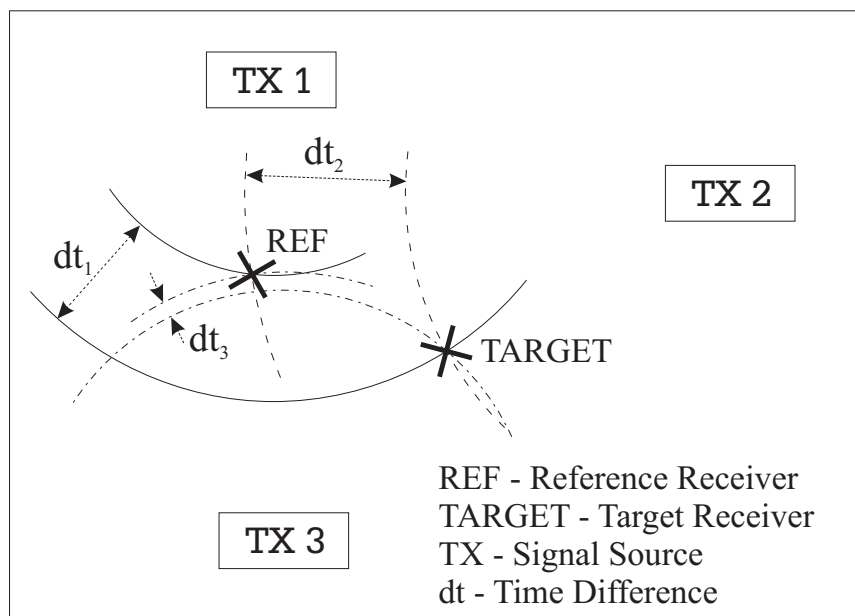
Figure 2.2: Illustration of TDOA System with Three Signal Sources
