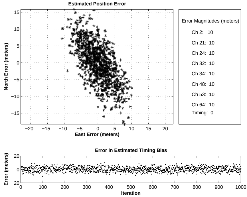
Figure 4.15: Simulated Position Estimation Error, 10 Meter Errors
