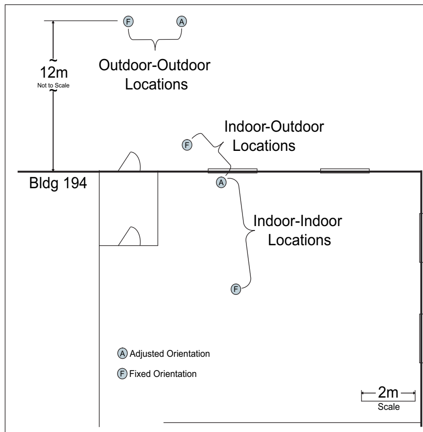
Figure 3.16: High Multipath Environment Test Diagram
