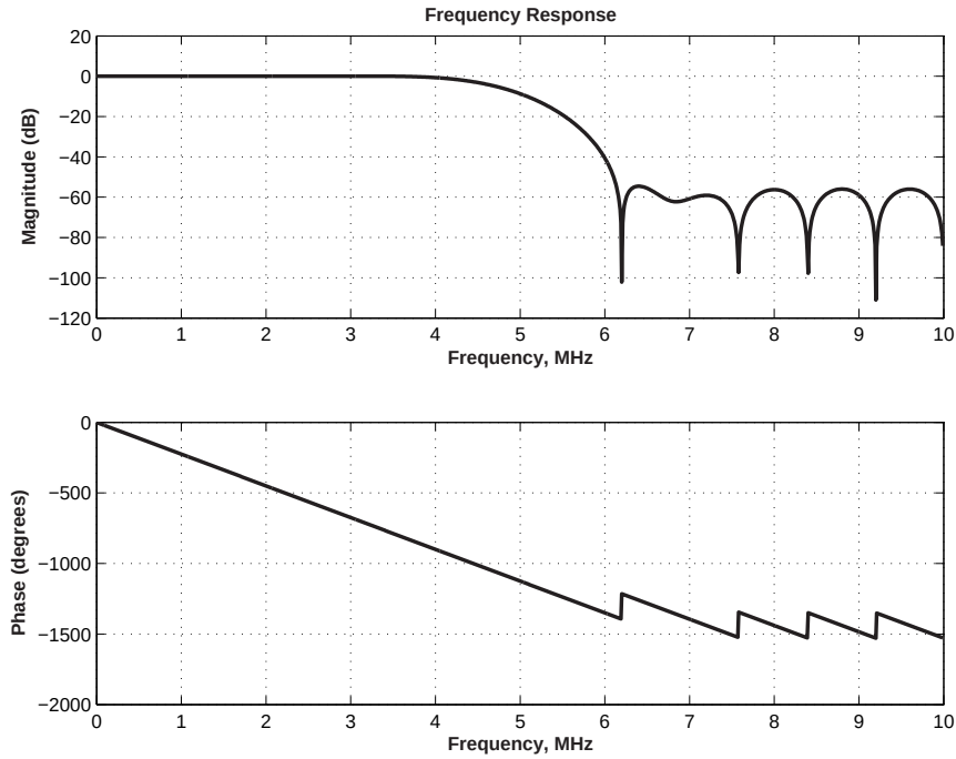
Figure 3.4: Magnitude and Phase Response of FIR Video Signal Filter
