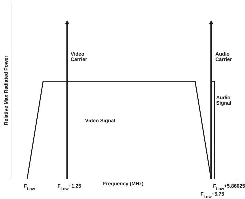
Figure 2.3: NTSC Bandwidth Allocations for a Particular Station
