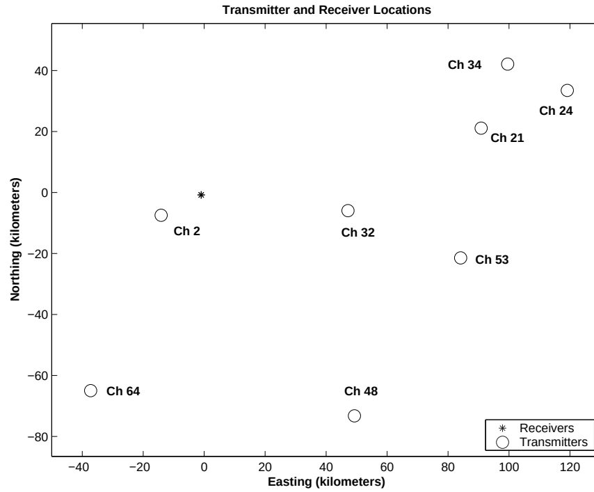
Figure 4.11: Expanded Dayton Area Television Transmitter Locations
