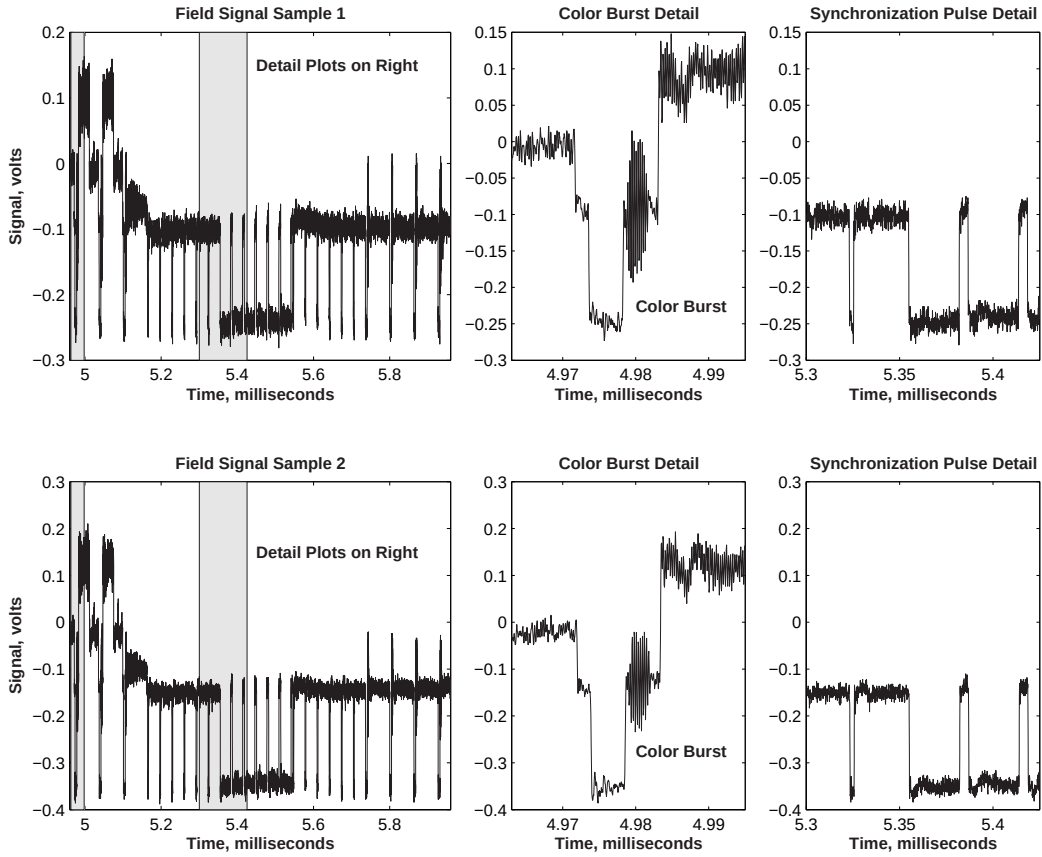
Figure 4.6: Field Signal Samples
