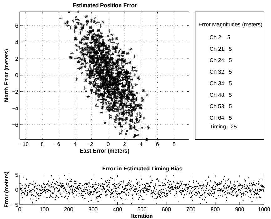
Figure 4.16: Simulated Position Estimation Error, 5 Meter Errors
