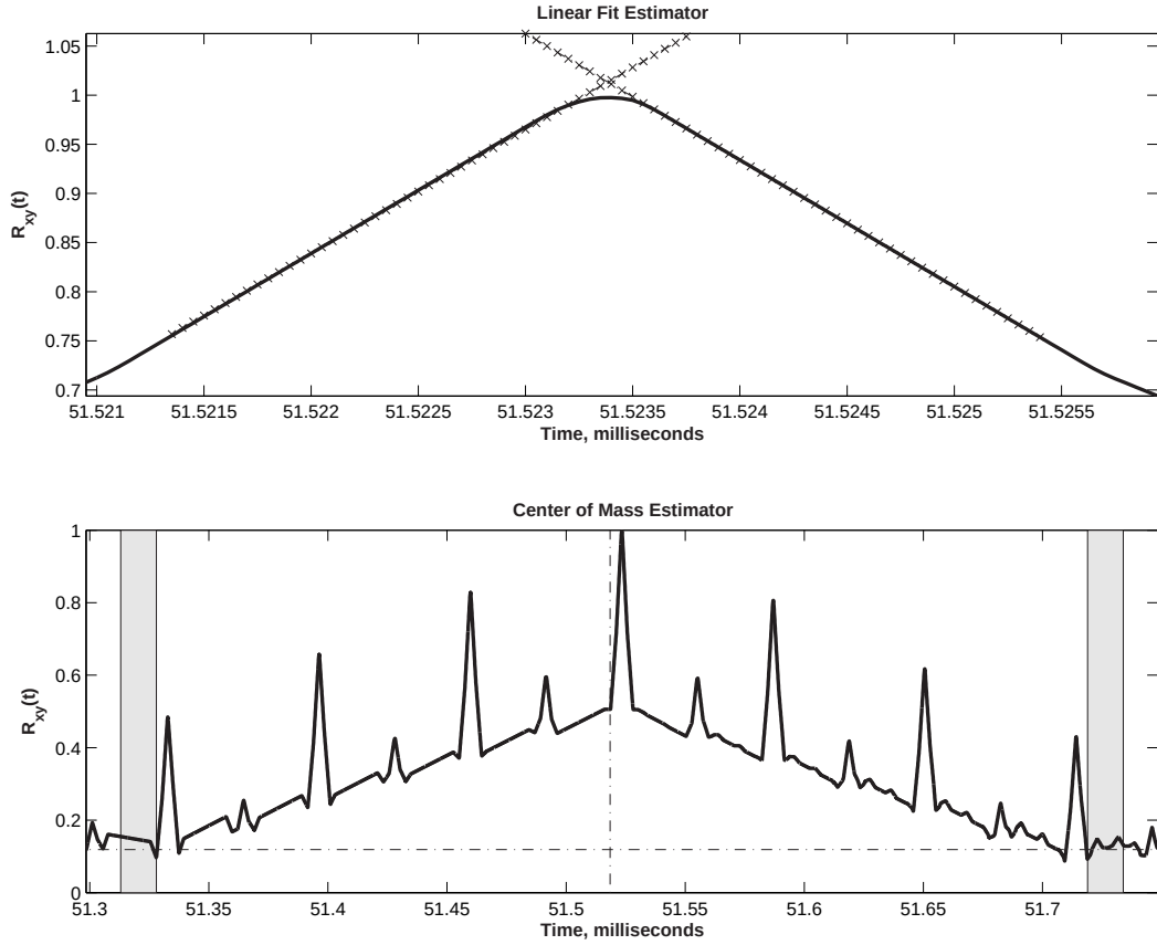
Figure 3.12: Illustration of Correlation Peak Estimators
