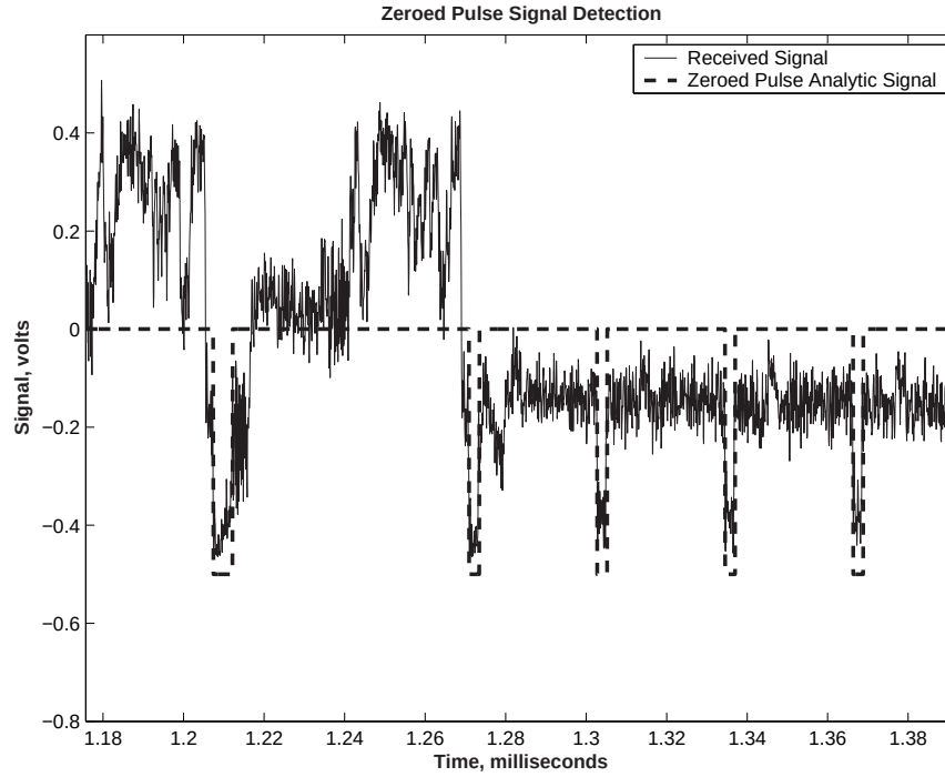
Figure 3.11: Zeroed Pulse Signal Detection
