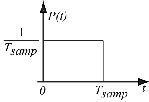
Figure 3.14: Probability Density of Discretization Error
