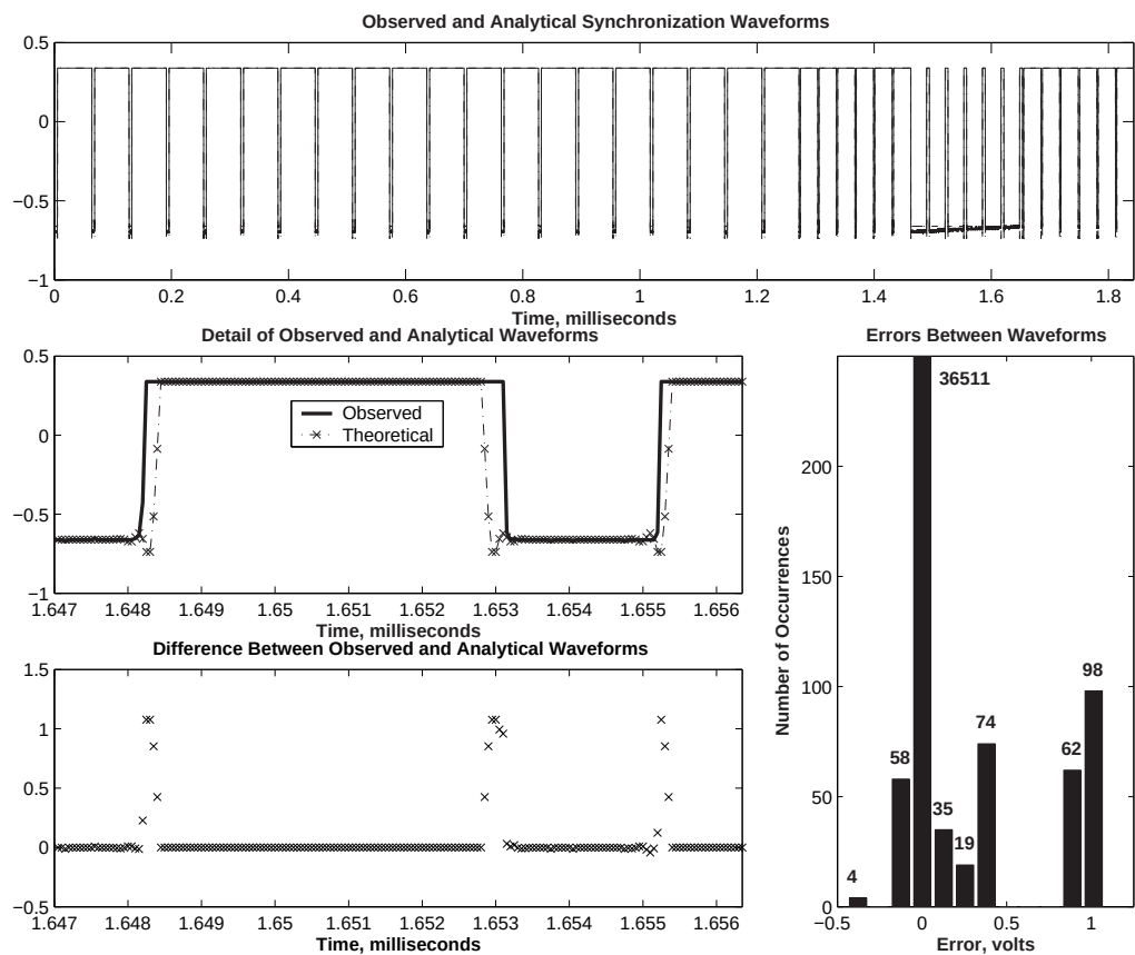
Figure 3.8: Timing Accuracy of the Analytical Model as Compared to the DVD Video Encoder
