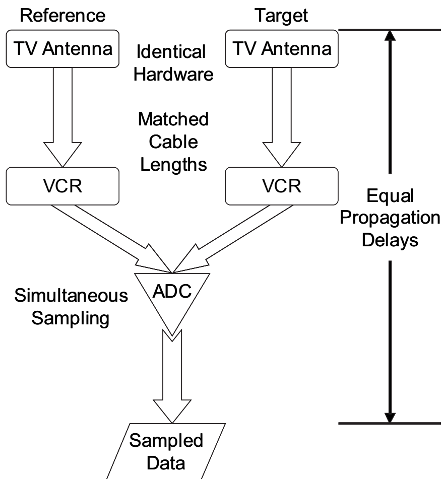
Figure 3.3: Signal Acquisition Flowchart
