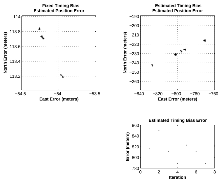
Figure 4.10: Dayton Four Station Position Estimation Error
