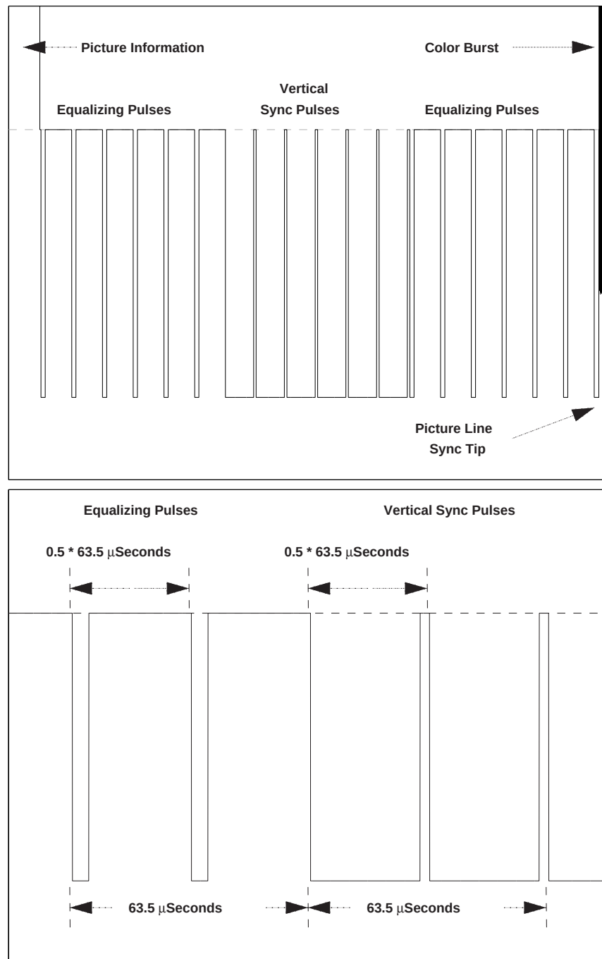
Figure 2.5: Upper: NTSC Synchronization Pulses Structure Lower: Synchronization Pulses Detail
