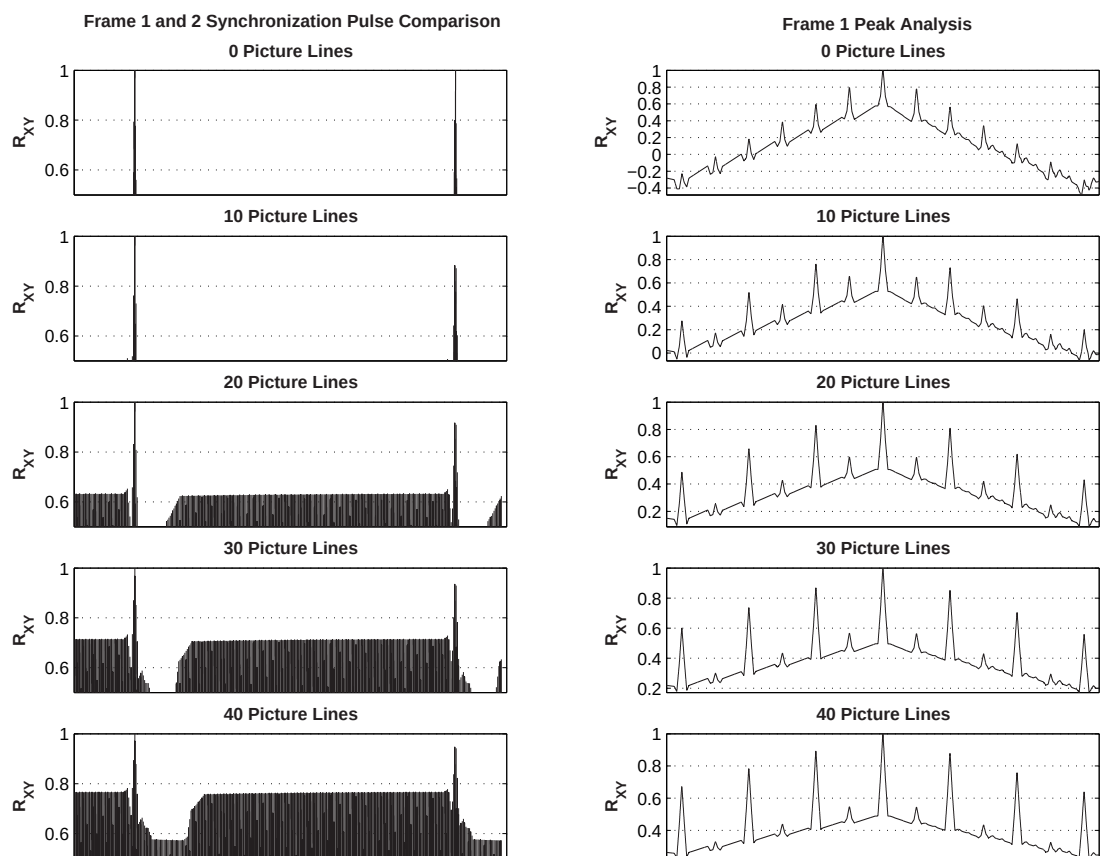
Figure 3.10: Waveform Development—Correlation Peak Analysis
