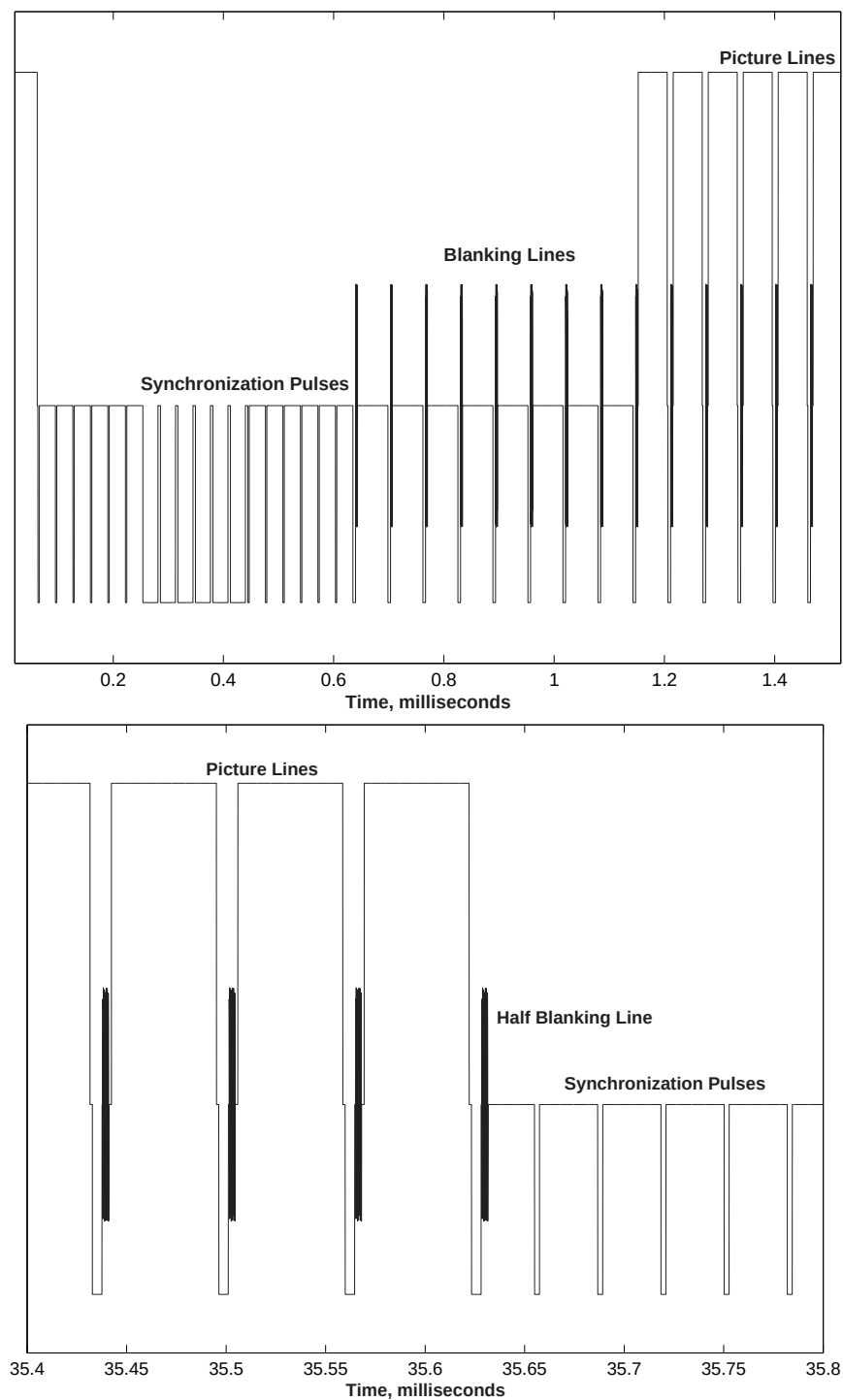
Figure 2.6: Upper: Video Signal with Frame 1 Synchronization Pulses Lower: Frame 2 Synchronization Pulses Offset
