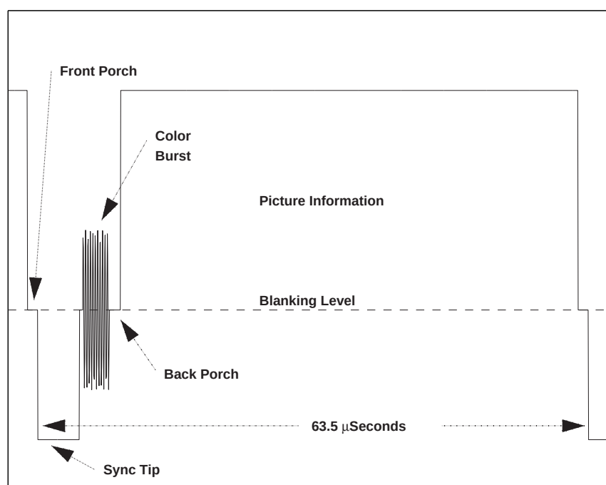
Figure 2.4: NTSC Picture Line Structure
