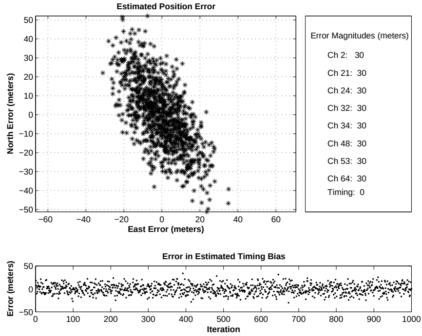
Figure 4.12: Simulated Position Estimation Error, Field-like Errors
