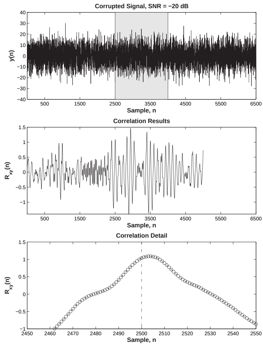
Figure 2.10: Correlation Results, SNR = -20 dB (Compensated to Indicate the Start of the Desired Signal)
