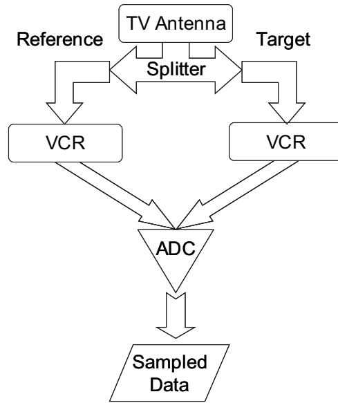
Figure 4.1: Zero Baseline Test Setup
