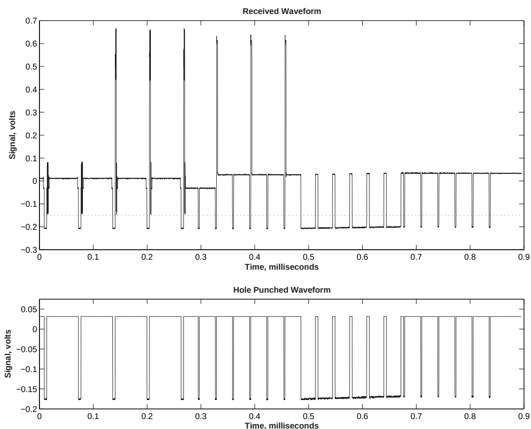
Figure 3.9: Example of Hole Punching Waveform
