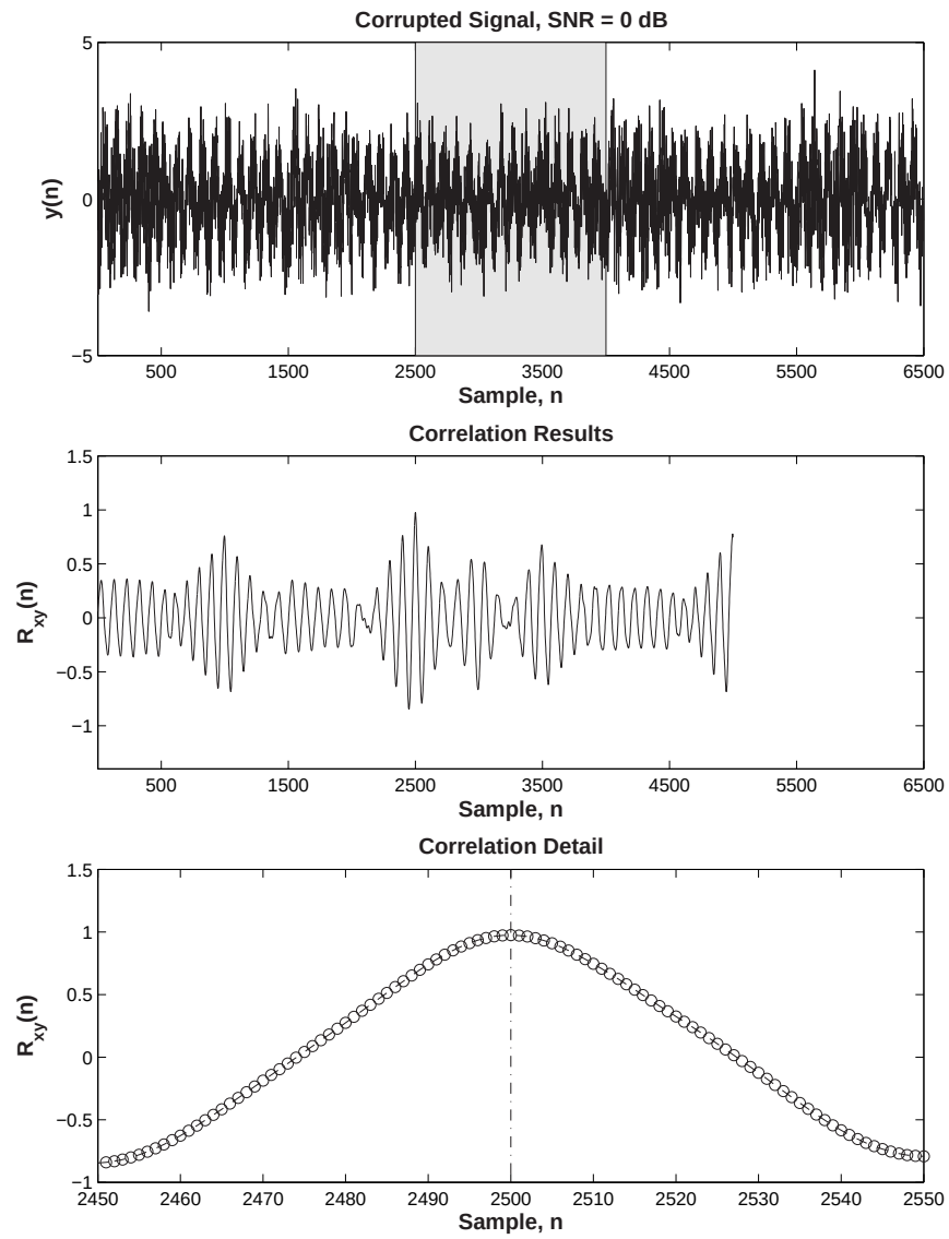
Figure 2.8: Correlation Results, SNR = 0 dB (Compensated to Indicate the Start of the Desired Signal)
