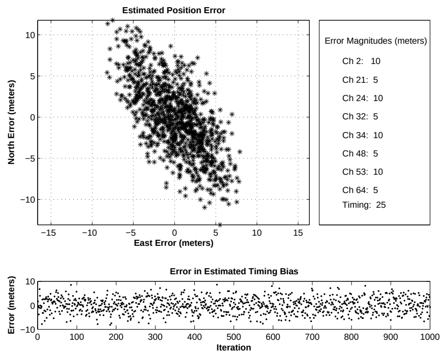
Figure 4.17: Simulated Position Estimation Error, Mixed 5 and 10 Meter Errors
