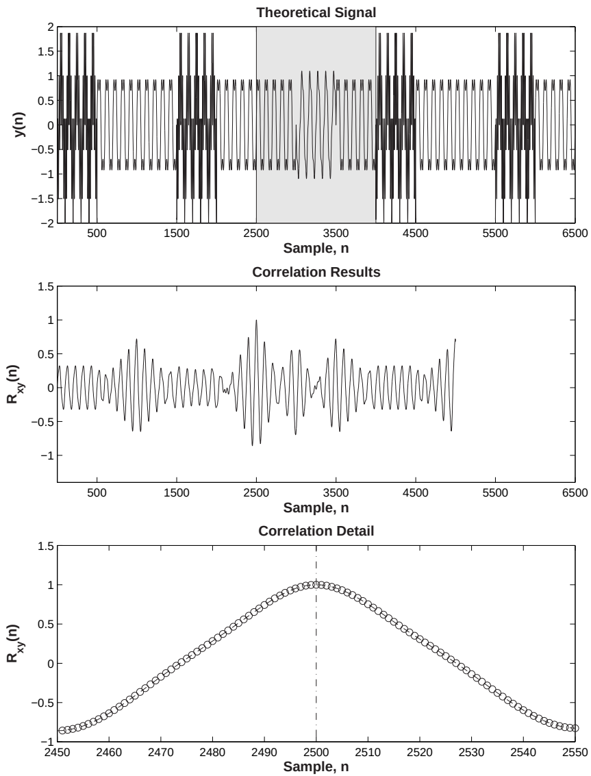
Figure 2.7: Correlation Results of Theoretical Signals (Compensated to Indicate the Start of the Desired Signal)
