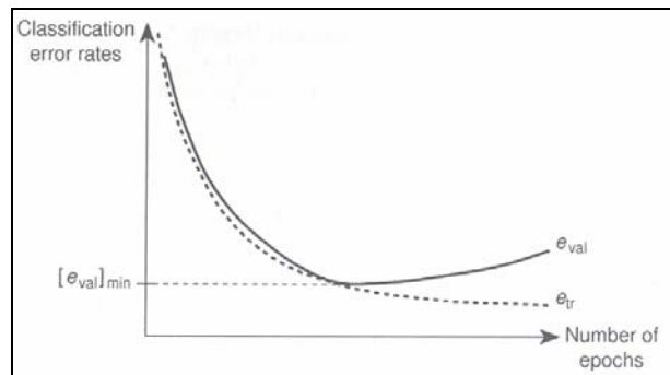
Figure 18 MLP NN Training Error Plot [39]
