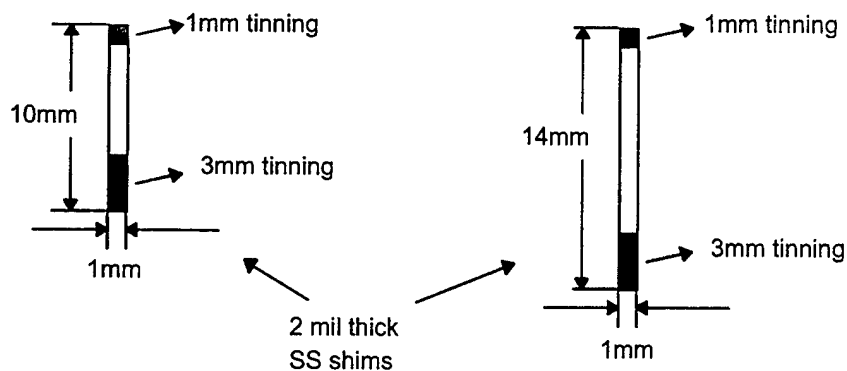
Figure 2-10. Schematic drawing of a pair of stainless steel shims.
