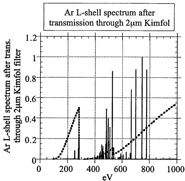
Figure 6-5. Ar L-shell spectrum as transmitted through the 2 \mu\text{m} Kimfol filter and the transmission of the Kimfol.
