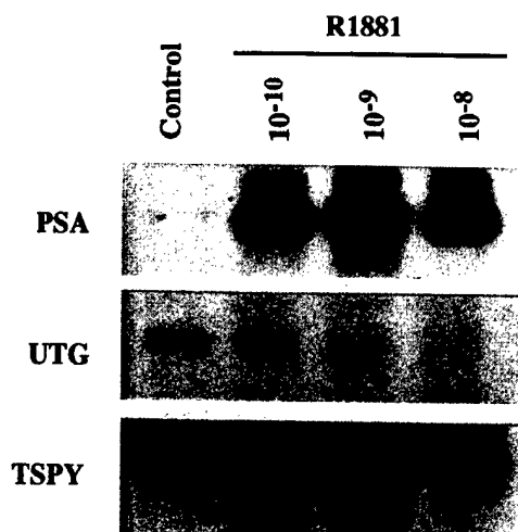
Figure 3. Northern blotting analysis of PSA , UTG , and TSPY transcripts in LNCaP cells treated with the synthetic androgen, R1881. PSA and TSPY steady state transcripts increased and those for UGT decreased under androgen stimulation of LNCaP cells.
