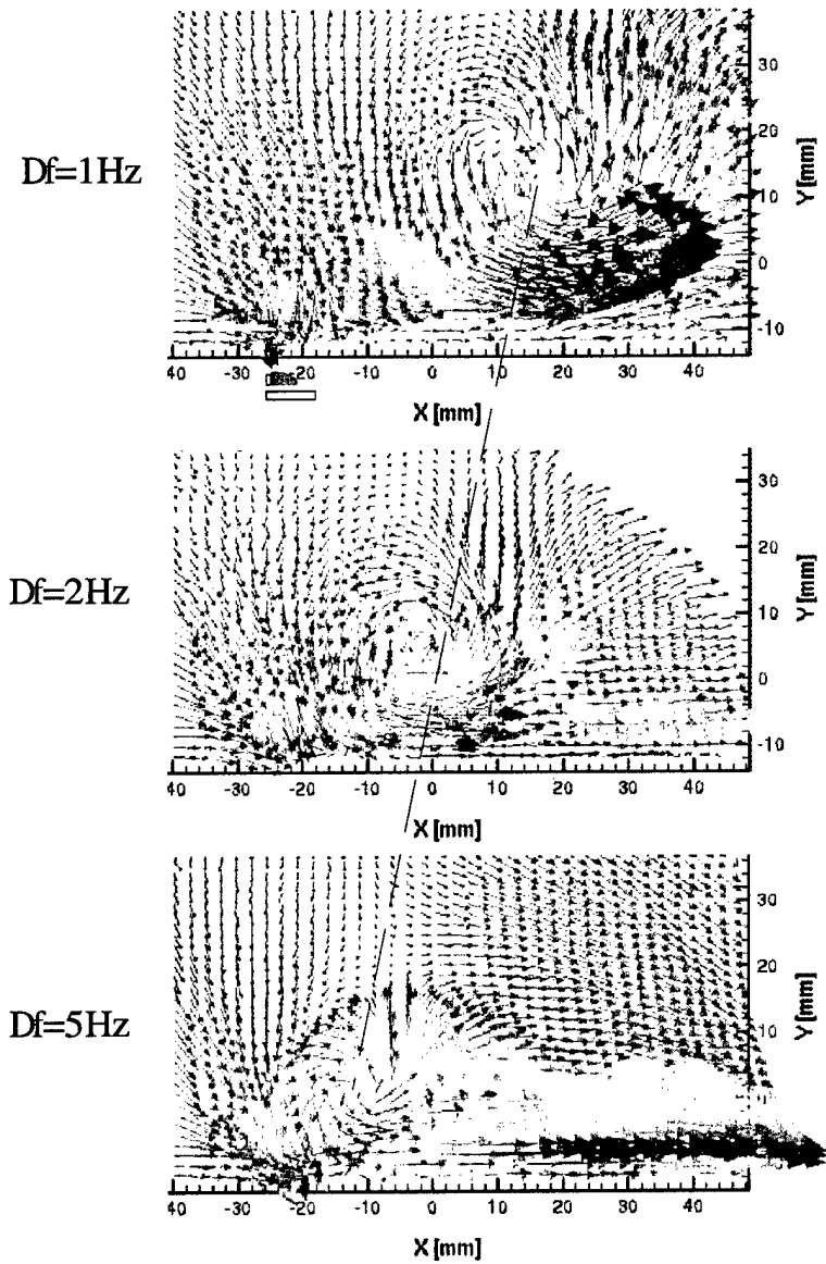
Figure 2.24. Phase-averaged velocity vectors at the same phase trigger, at different frequencies of the plasma actuator.
