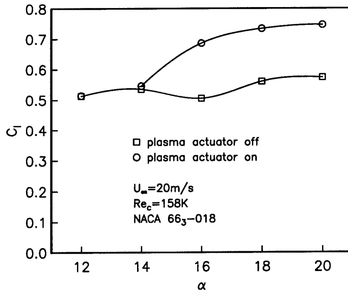
Figure 4.11. Comparison of lift coefficient versus angle of attack on the NACA 66 3 - 018 airfoil with the plasma actuator off and on at Re_c = 158K .
