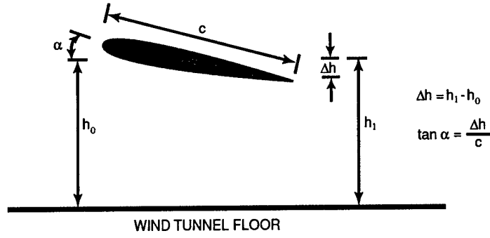
Figure C.2. Geometric relationship between airfoil and the test section floor.
