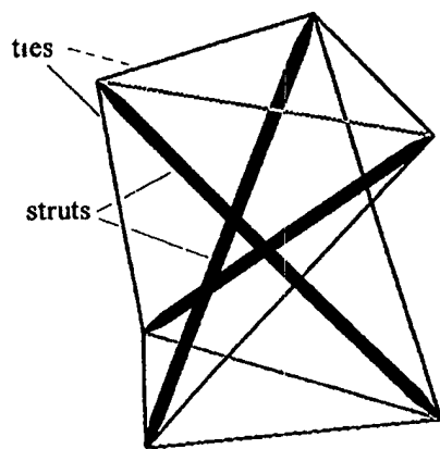
Figure 1 Tensegrity Prism
