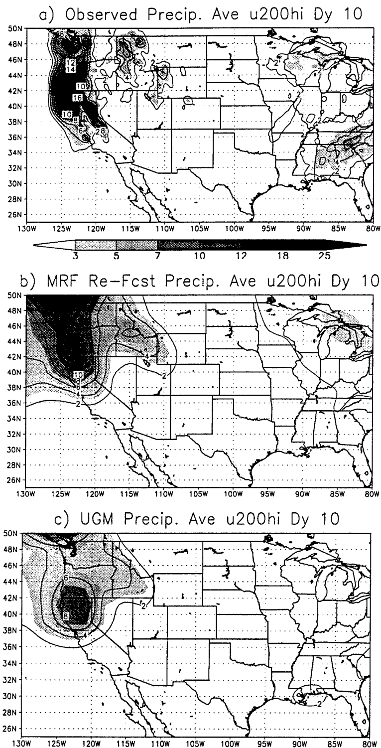
FIG. 9. Composite of average day 10 precipitation accumulation (cm) of u200hi years (1996 and 2000). (a) Observed u200hi precipitation (Higgins et al., 1996). (b) MRF u200hi precipitation. (c) Uniform resolution UGM, u200hi precipitation. The contour interval is 2 cm (contouring in (a) is up to 20 cm), and shading is for accumulation greater than or equal to 3 cm. The maximum observed accumulation in (a) is 24 cm.
