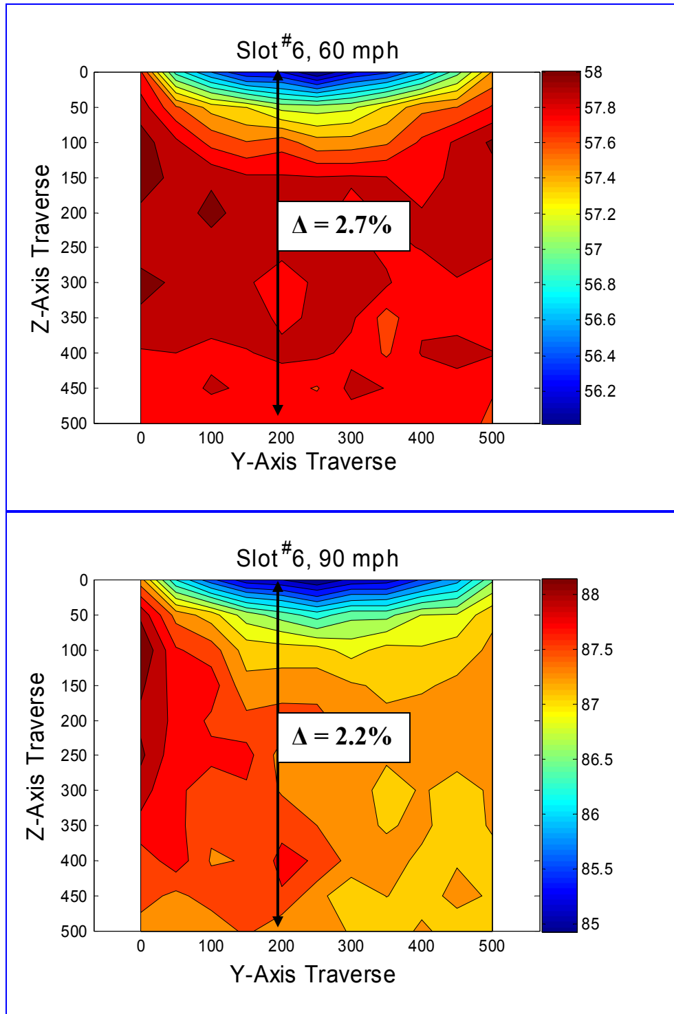
Figure 51. Slot #6 U_{\text{Mean}} Velocity Contour Plots
