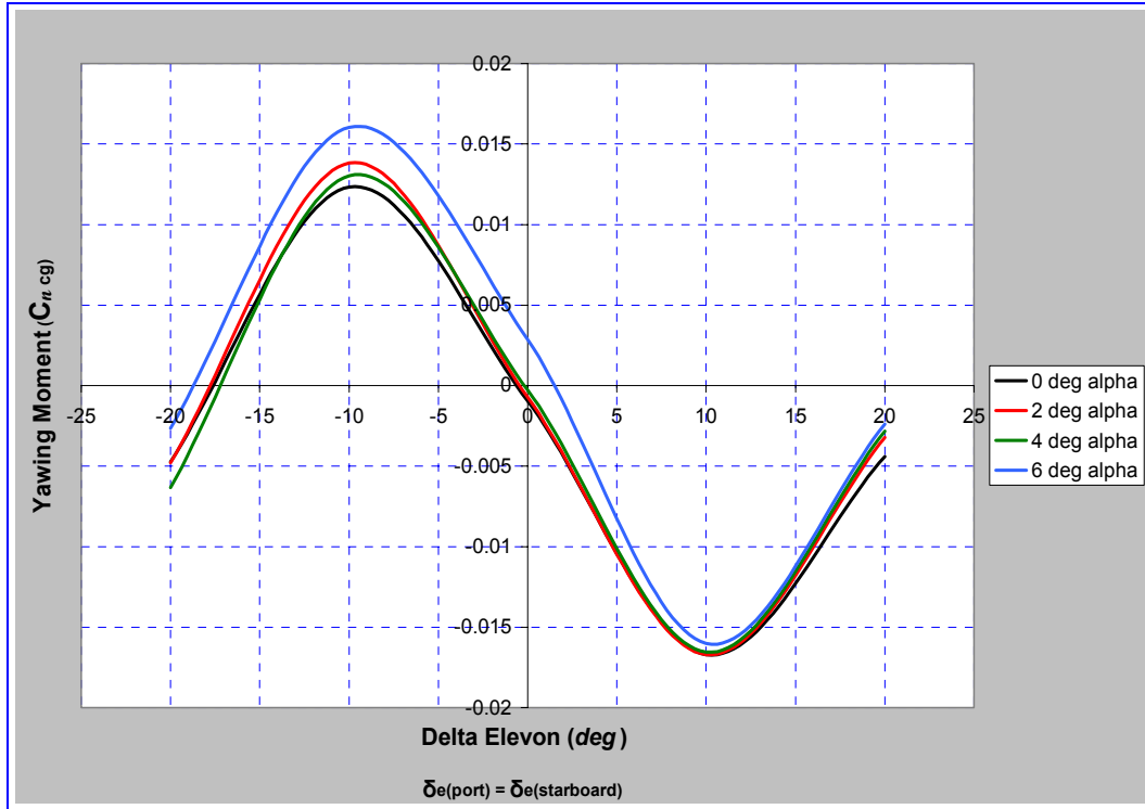
Figure 37. Flex Wing MAV C_n vs. \delta_{\text{Elevon}} (Tandem)
