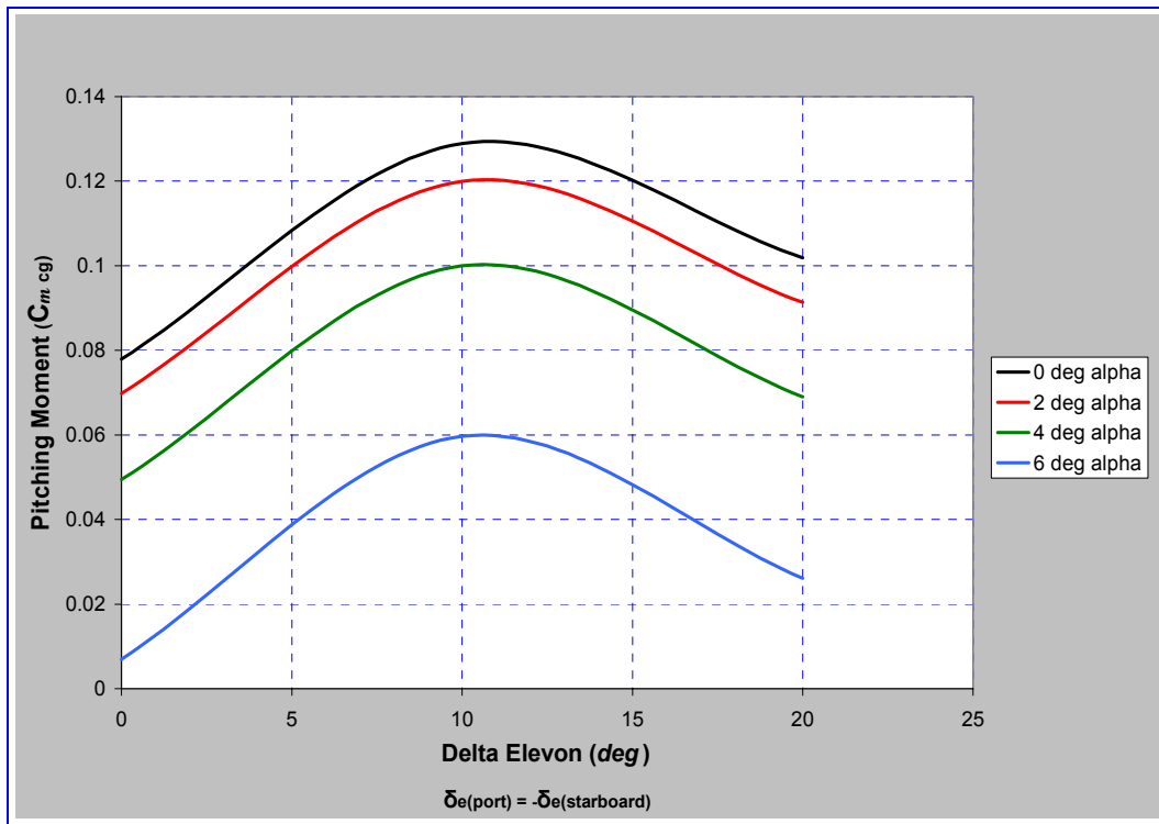
Figure 38. Flex Wing MAV C_m vs. \delta_{\text{Elevon}} (Opposed)
