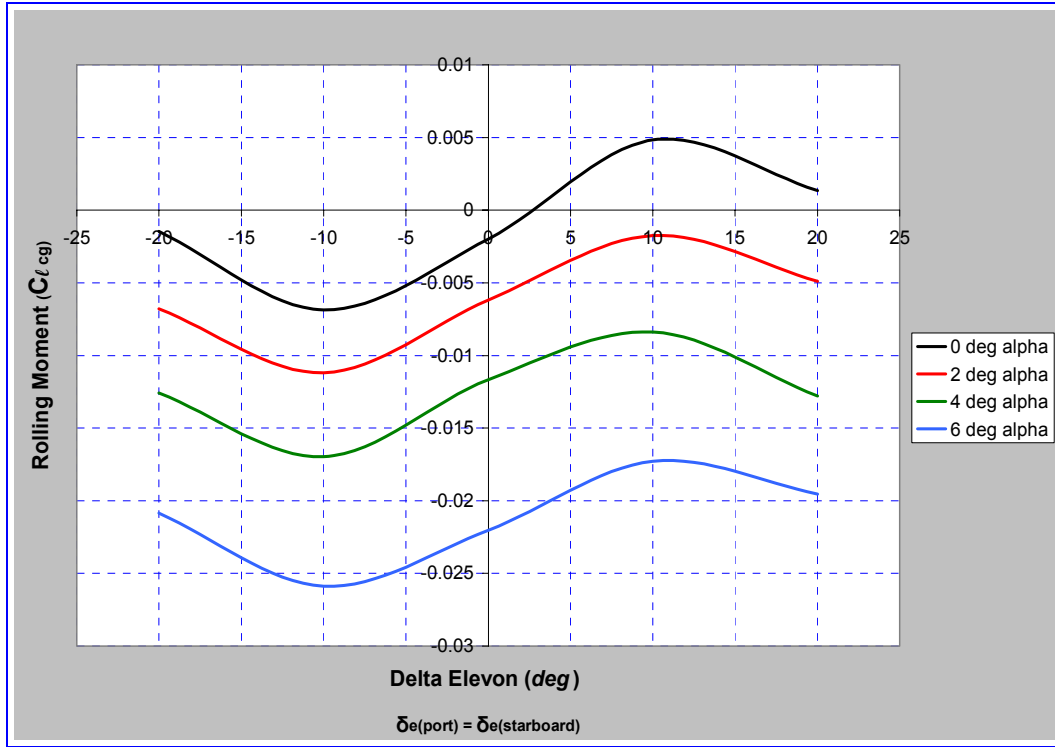
Figure 36. Flex Wing MAV C_l vs. \delta_{\text{Elevon}} (Tandem)
