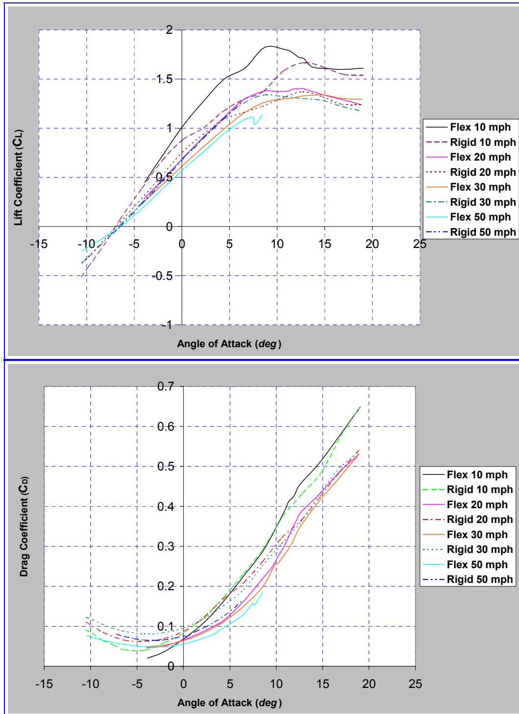
Figure 18. Flexible and Rigid Wing MAV C_L vs. \alpha and C_D vs. \alpha
