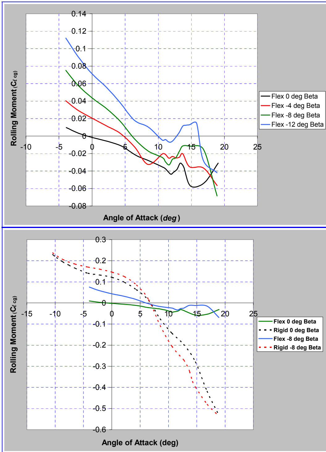
Figure 26. Flexible and Rigid Wing C_l vs. \alpha for Various Angles of \beta
