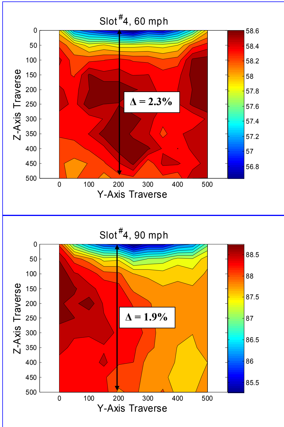
Figure 50. Slot #4 U_{\text{Mean}} Velocity Contour Plot
