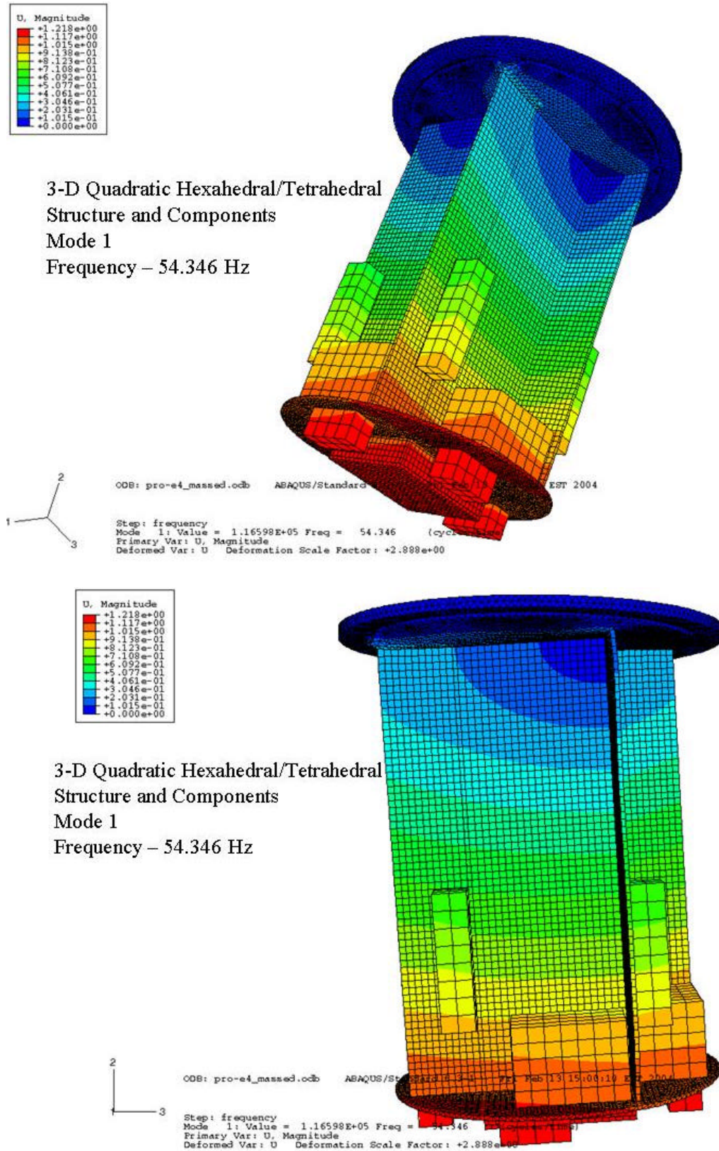
Figure 44. Mode 1 for the Massed Three-Dimensional Model of the RIGEX Structure
