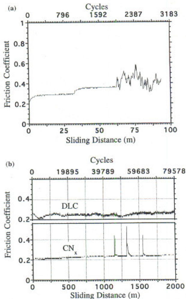
Fig. 13. Friction coefficient as a function of total sliding distance of: (a) a CN x film deposited without a Ti interlayer; and (b) CN x and DLC films deposited with a Ti interlayer.
