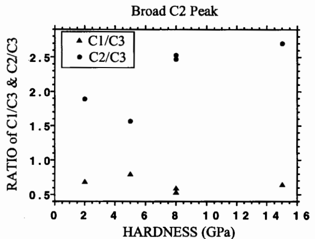
Fig. 10. Ratios of carbon (1s) integral intensity obtained from XPS, C1/C3 and C2/C3, as a function of film average hardness for films with C2 peak width = 2.22–3.05 eV.
