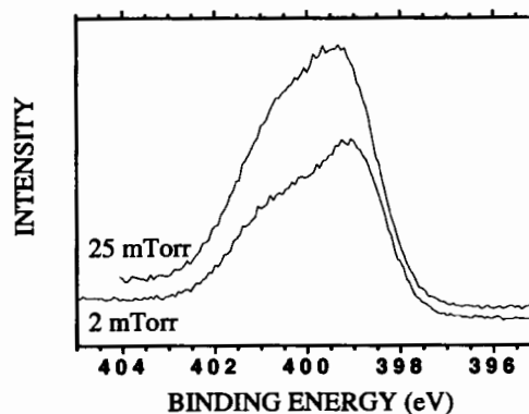
Fig. 6. Nitrogen (1s) spectra obtained from CN_x film deposited at 2 and 25 mtorr nitrogen, d = 8 cm, 200 W ECR power, 100 W magnetron power, and substrate at floated condition.
