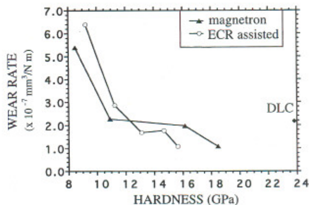
Fig. 15. Variation of wear rate with film hardness. Data were obtained from 1000-m sliding tests of CN x and DLC films that were deposited with a Ti interlayer.
