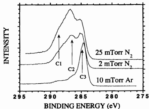
Fig. 7. Carbon (1s) spectra obtained from a DLC film deposited at 10 mtorr Ar, 400 W magnetron power, and CN_x film deposited at the same conditions as those shown in Fig. 6.
