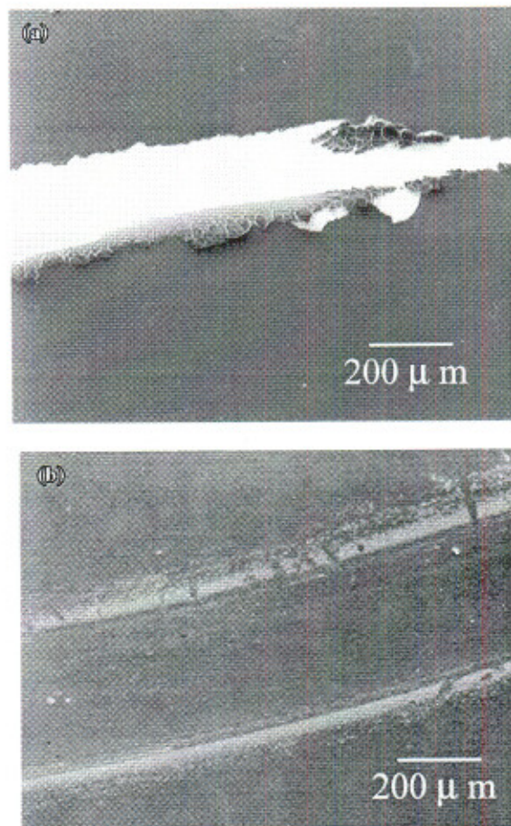
Fig. 14. SEM micrograph of wear track surface obtained from the CN x film coated 440C disc after the unlubricated ball-on-disc test, shown in Fig. 13: (a) without a Ti interlayer; and (b) with a Ti interlayer.
