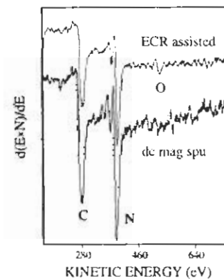
Fig. 4. Typical Auger spectra of CN_x films deposited with and without ECR assistance.
