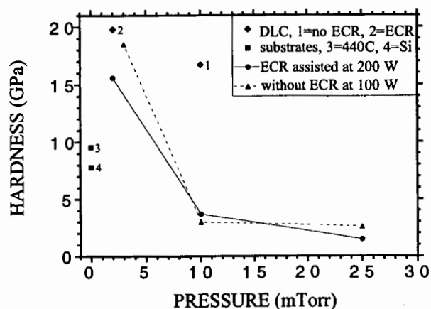
Fig. 11. Average hardness of CN_x films deposited without and with ECR (200 W) assistance. The films were deposited at 100 W target power and 8 cm substrate-to-target distance.
