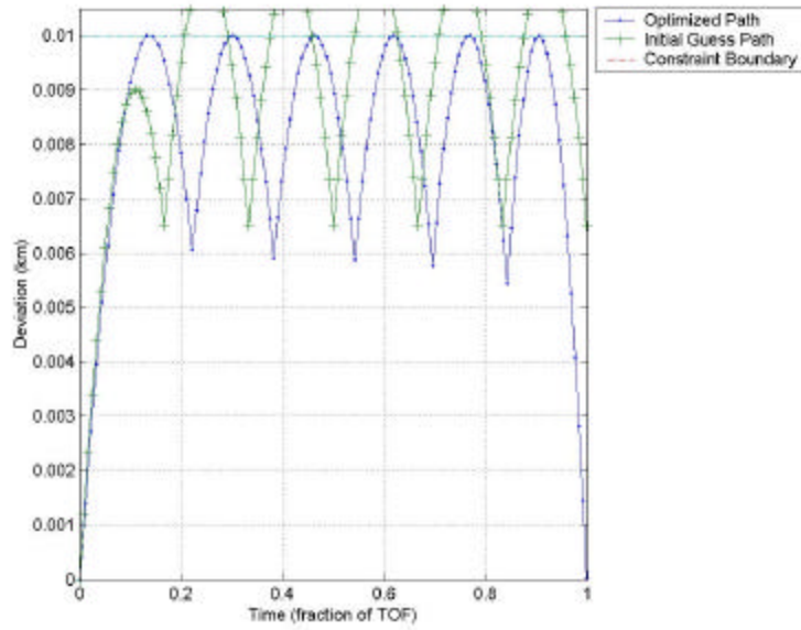
Figure 21. Deviation of Initial Guess Radius = 6.5 m and b = 6 . \Theta_y=90^\circ , \Theta_z=0^\circ , \gamma_0=45^\circ with TOF = 0.1 and \rho_{\max}=0.01 km
