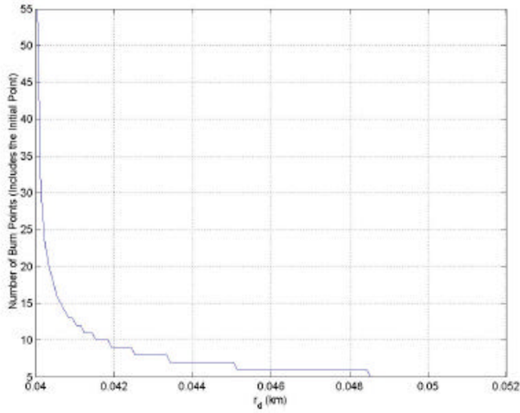
Figure 26. Number of Burn Points vs. r_d . \Theta_y = 90^\circ , \Theta_z = 0^\circ , \gamma_0 = 45^\circ with TOF = 0.1 and \rho_{\max} = 0.01 km
