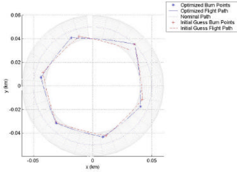
Figure 20. Initial Guess Radius = 6.5 m and b = 6 . \Theta_y=90^\circ , \Theta_z=0^\circ , \gamma_0=45^\circ with TOF = 0.1 and \rho_{\max}=0.01 km
