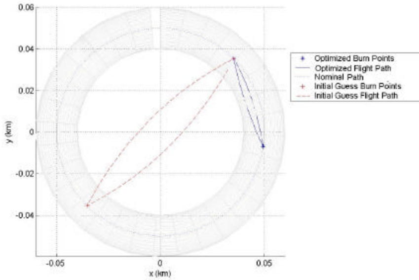
Figure 11. Two Burn Points. \Theta_y=90 , \Theta_z=0 , \gamma_0=45 with TOF = 0.1 and \rho_{\max}=0.01 km
