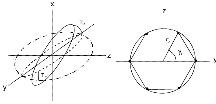
Figure 1 a) Rotated Nominal Path b) Unrotated Nominal Path
