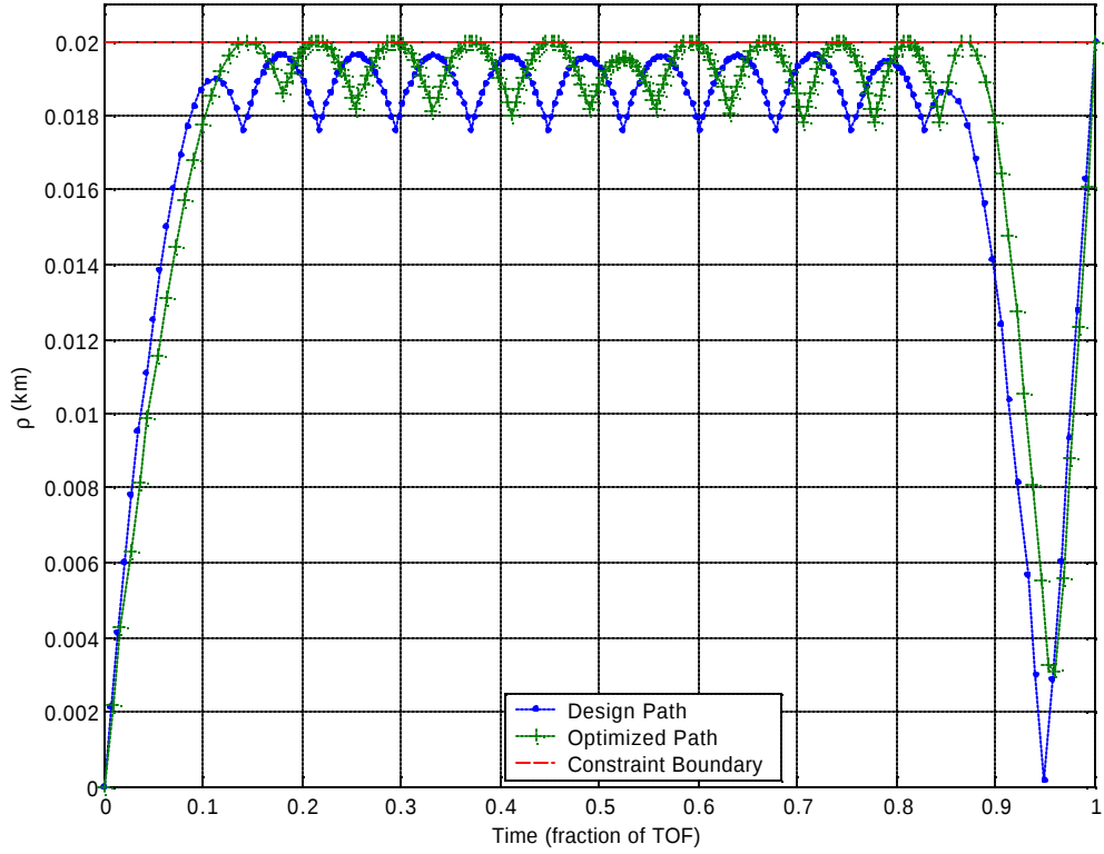
Figures 34. Design and Optimized Circumnavigation Path Deviations— Larger r_0 . r_0 = 100 m, \Theta_y = 60^\circ , \Theta_z = 30^\circ , \gamma_0 = 45^\circ with TOF = 0.1 and \rho_{\max} = 0.02 km
