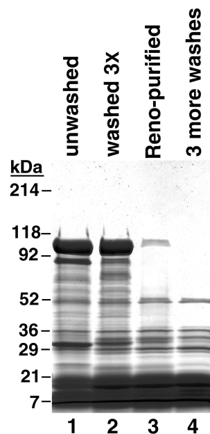
FIG. 3. Levels of contaminating EA1 at selected stages of purification of B. anthracis spores. For each stage, a sample containing the same number of spores was treated to extract spore surface proteins, and these proteins were separated by SDS-PAGE and visualized by Coomassie blue staining. EA1 levels were measured after spores were harvested (lane 1), after spores were washed three times (lane 2), after spores were sedimented through 50% Renografin (lane 3), and after spores were washed three more times (lane 4). The position of EA1 in the gel is marked with a filled arrowhead.
