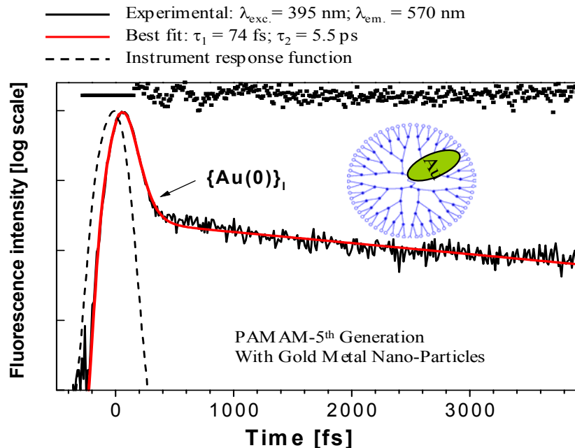
Figure 4: The dynamics of the emission decay measured by fluorescence upconversion spectroscopy. The decay curve suggested that the principle emission is a fast component on the order of \sim 80 \text{ fs} and a slower component (several ps). We have attributed the fast component to the emission of the metal nanoparticles in the dendrimer host.
