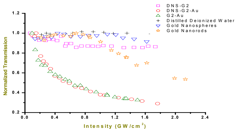
Figure 2: Nonlinear transmission results for a comparison of different metal topologies as well as dendrimer metal nanocomposite morphologies. Both gold nanorods and nanospheres were measured (at 532 nm, ns pulses) as well as gold dendrimer nanocomposites and a functionalized chromophore dendrimer metal nanocomposite. The result suggests that while the mechanism of the nonlinear transmission effect in these systems does involve the metal nanoparticle, this effect is enhanced by the dendrimer architecture as well as in the functionalized chromophore.
