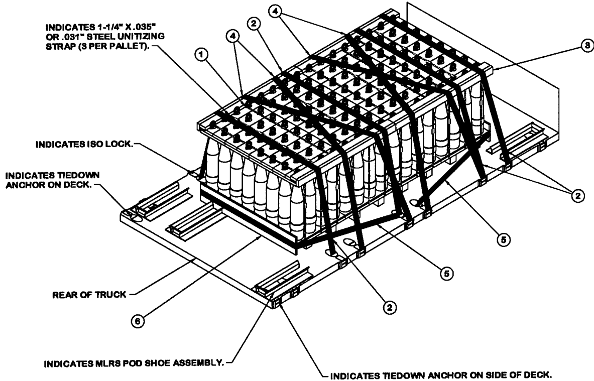
ISOMETRIC VIEW
