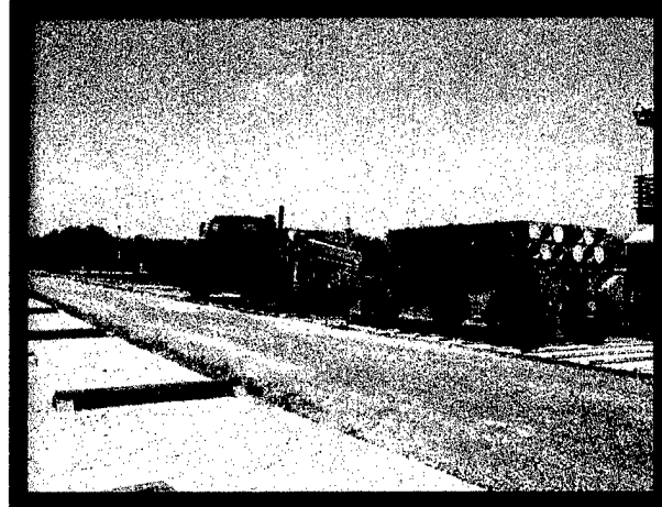
Photo 4. Washboard Course Testing of the RSV and RST with 2 Pods
