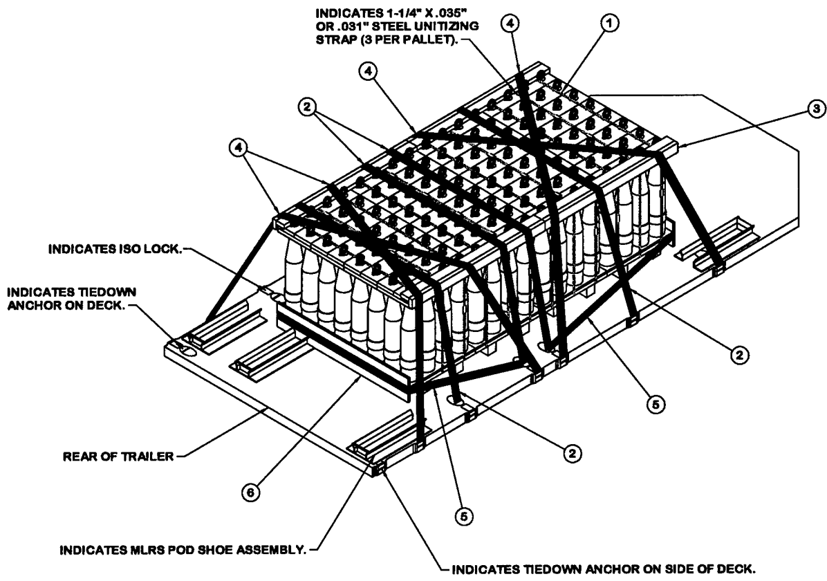
ISOMETRIC VIEW
