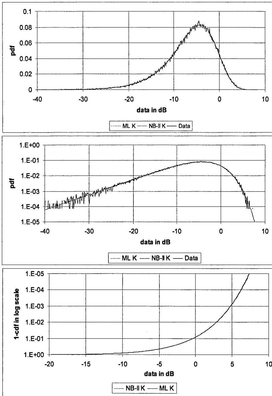
Figure 10: Comparison of parameter estimation schemes for the K-distribution using the AirSAR single-look L-band VV clutter data of homogenous open forests.
