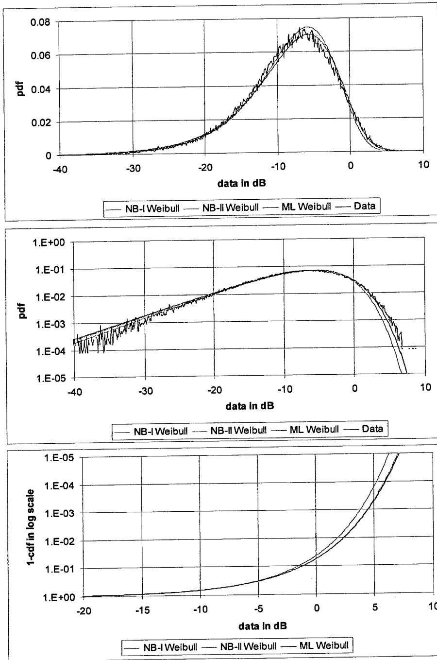
Figure 12: Comparison of the estimation schemes for the Weibull distribution using the AirSAR single-look C-band VV data of heterogenous clutter. The NB-I estimates are not as good as the NB-II estimates.
