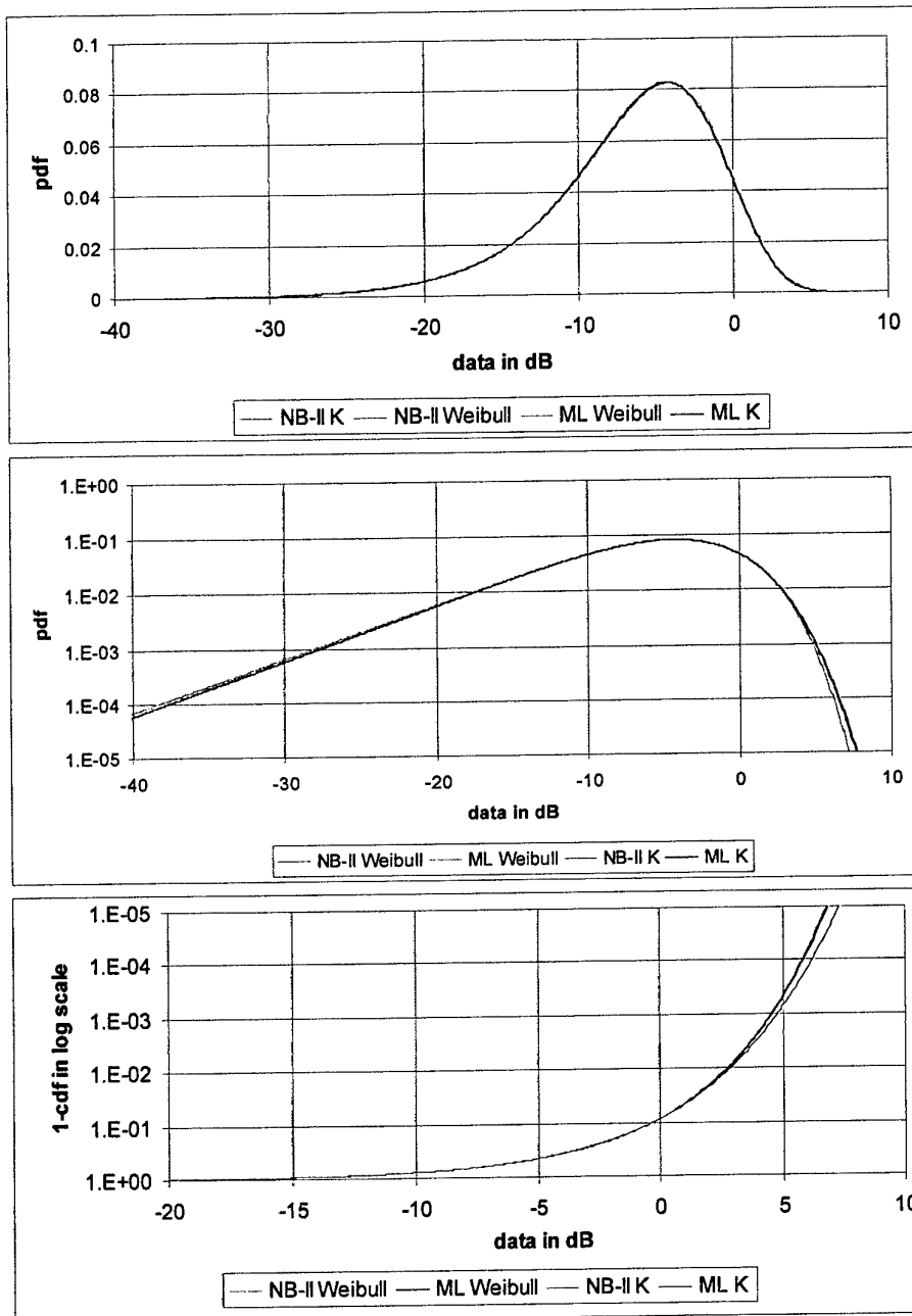
Figure 11: Comparison between the Weibull and the K- distributions for the AirSAR L-band VV clutter of homogenous open woodland of native eucalyptus. Both the ML estimates and the NB-II estimates provide the nearly identical pdf and cdf for the Weibull and the K-distributions, respectively. The convergence of the K-distribution is a little bit slower.
