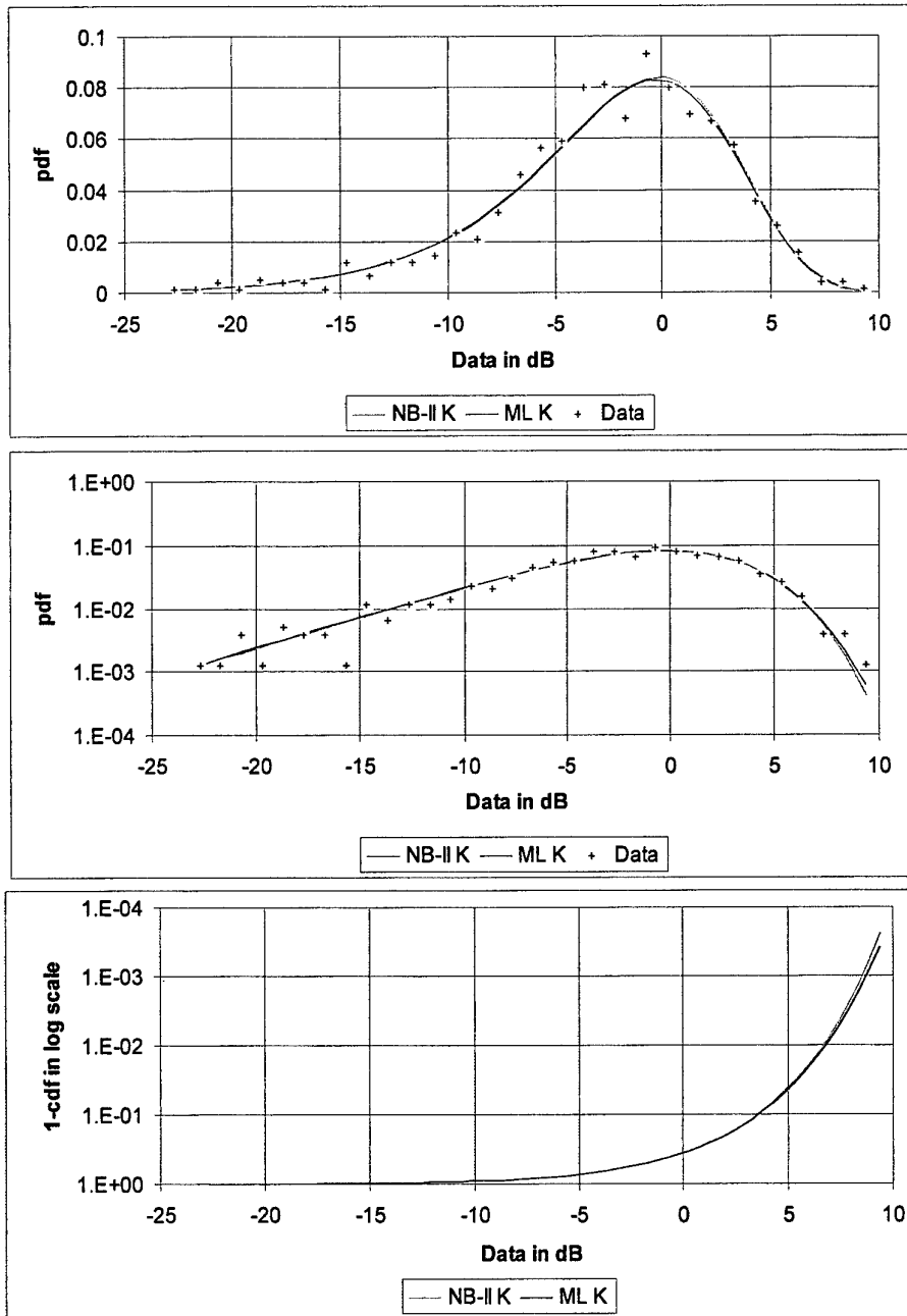
Figure 7: Comparison of parameter estimation schemes for the K-distribution using the MCARM RAR L-band VV clutter data of homogeneous farmland.
