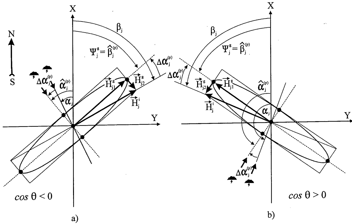
Fig.3.2.3. Formation of elliptic polarization in the gyrotronic Earth-ionosphere cavity:
