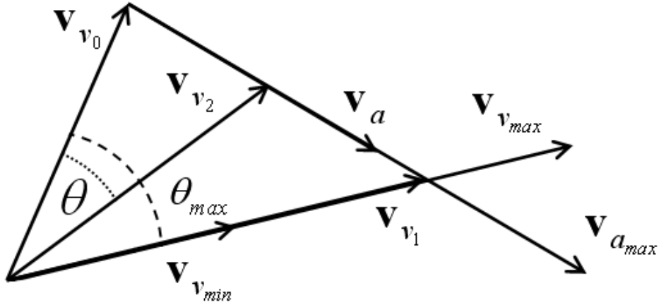
Figure 10 Visual depiction of vectors and actuator constraints associated with vehicle movement
