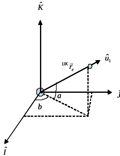
Figure 5- Relationship between \hat{u}_1 and IJK Coordinate Frame
