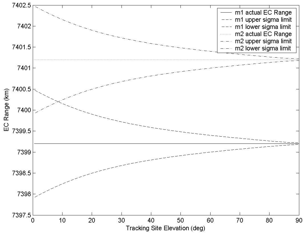
Figure 3- Affect of Elevation Angle on s_r
