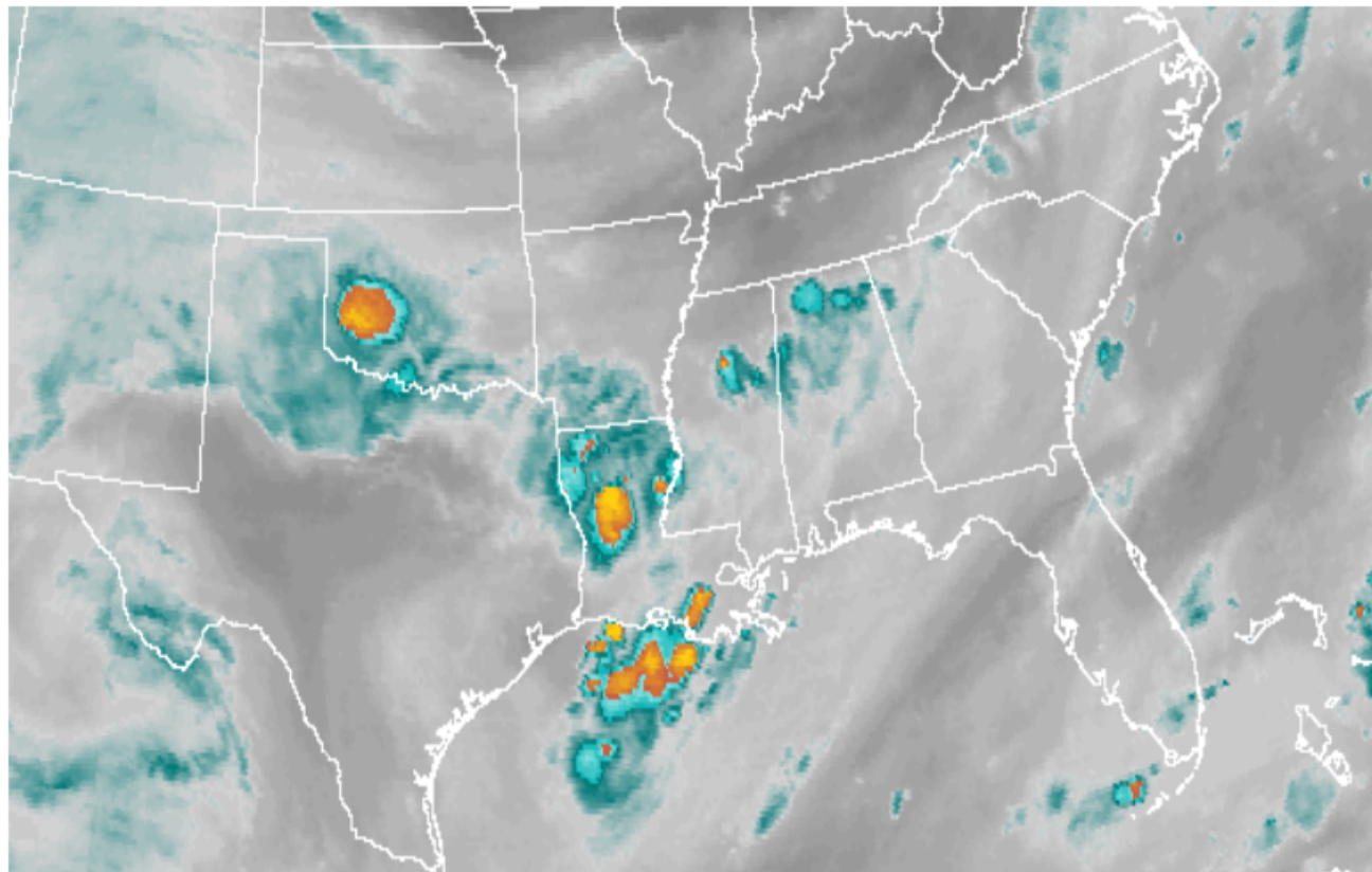
Figure 4.6. Water Vapor.
