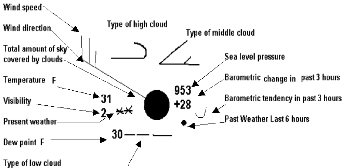
Figure 2.6. Station Model.
