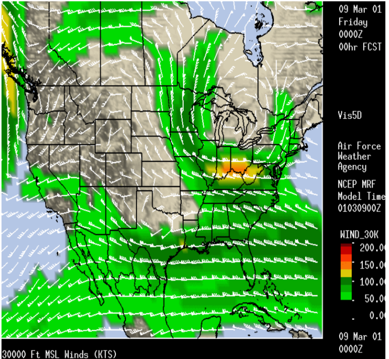
Figure 2.9. 30,000 ft Winds.
