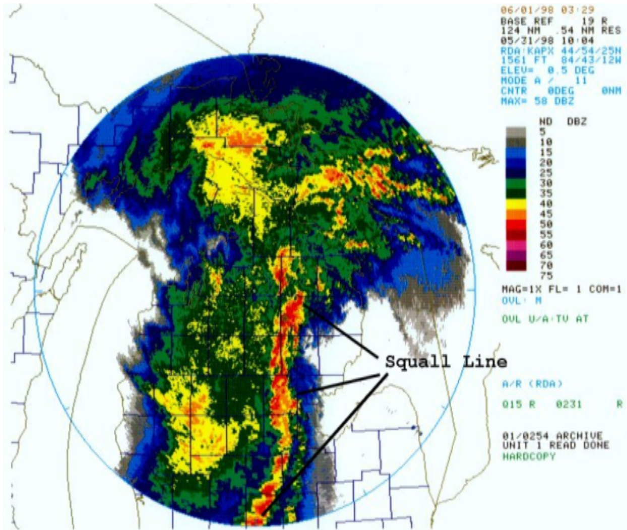
Figure 5.8. Squall Line.
