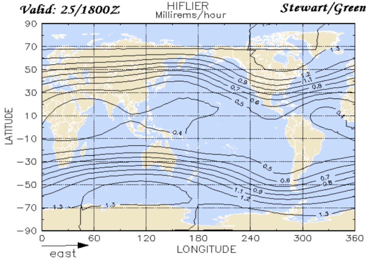
Figure 7.4. Space Impacts.
