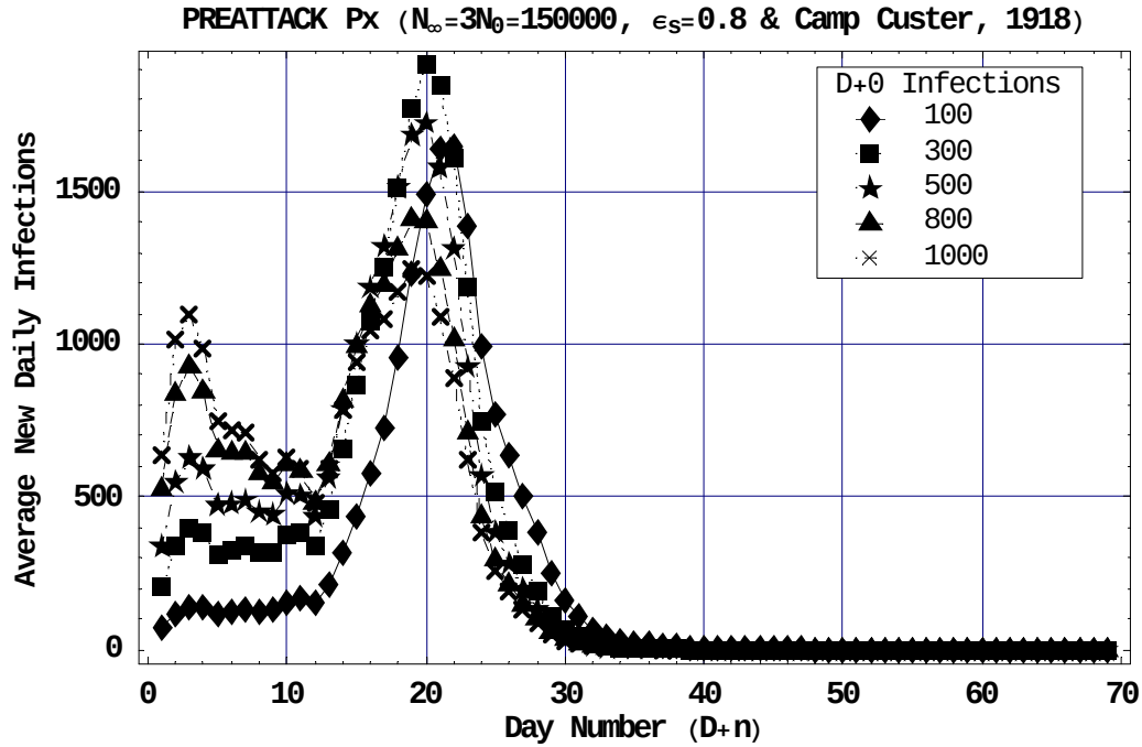
Figure 39. Estimated Average New Daily Infections for a Time-Dependent Vaccinated Population Emulating the Spread of Influenza from a U.S. Military Base into the Surrounding Civilian Community
