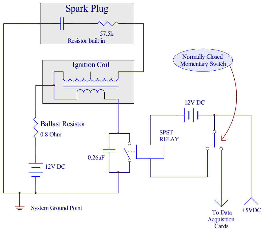
Figure 8. Ignition Circuit
