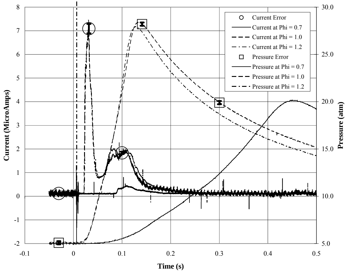
Figure 15. Effects of \phi = 0.7, 1.0, \& 1.2 at initial pressure of 5 atm
