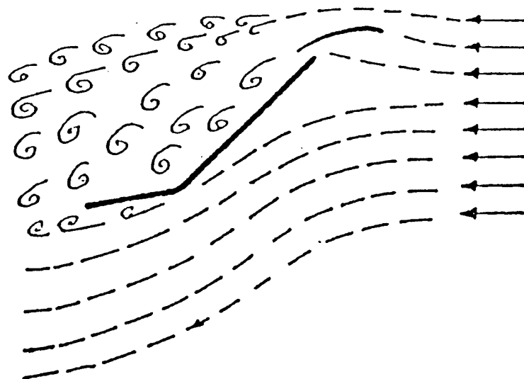
a) Schematic of flow over a reconfigured swept wing at 45^\circ incidence indicating fully separated flow.
