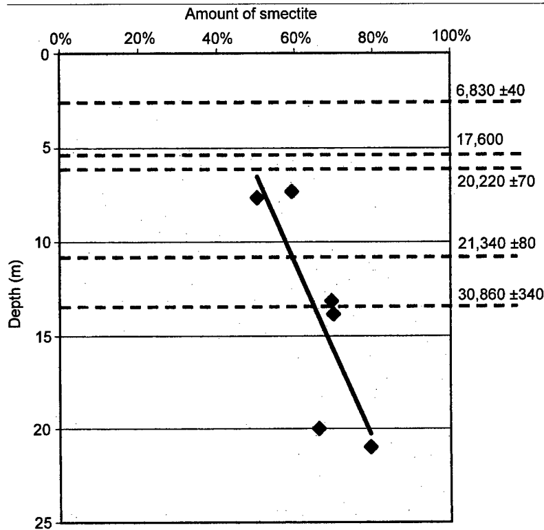
Figure 6. Percent smectite in Core RW2, Rosamond West Beach Ridge. The horizontal dashed lines represent AMS radiocarbon ages shown in the right-hand margin.
