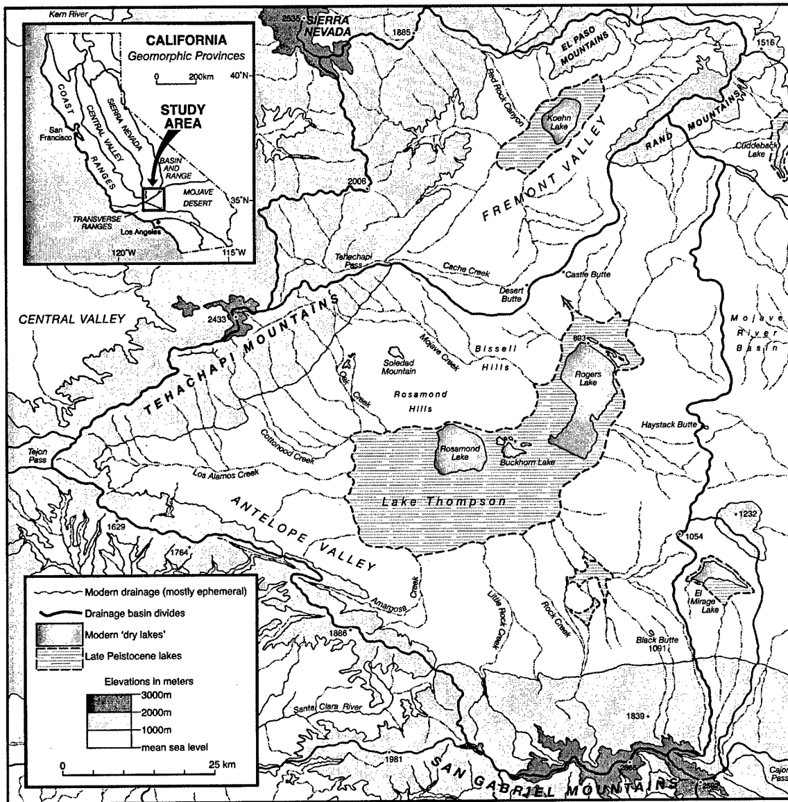
Figure 1. Lake Thompson in its regional setting.
