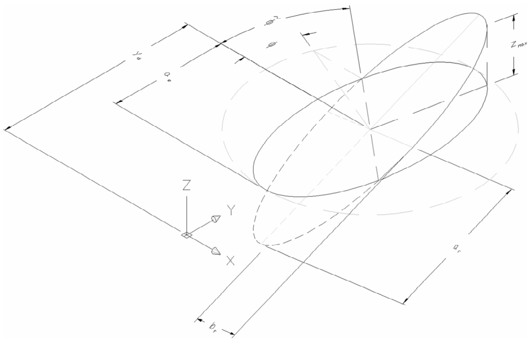
Figure 3.11 First-Order Force-Free Stationary Formations: 3-D View
