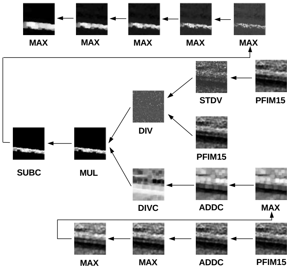
Figure 3.5. Feature images output by the nodes of the best composite operator from smart GP.
