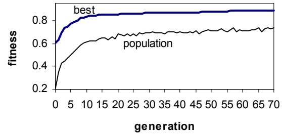
Figure 2.23. Fitness versus generation (person).
