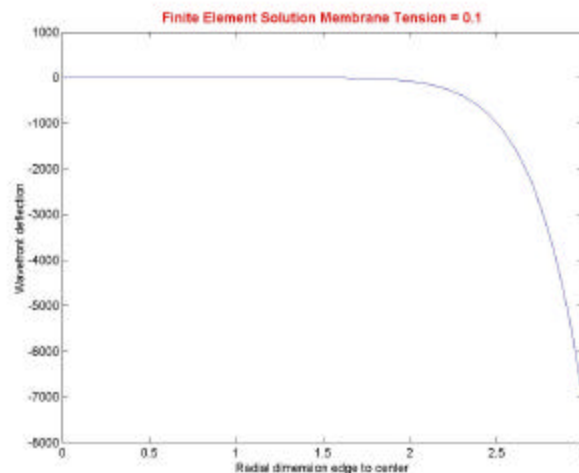
Figure 40. Membrane Deflection (N=0.1)
