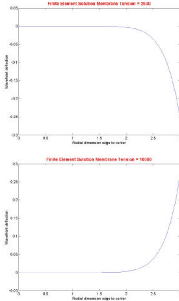
Figure 42. Membrane Deflection (N=2500, 10,000)
