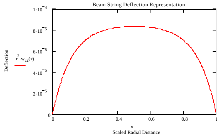
Figure 21. Beam String Deflection ( N_0=5 )
