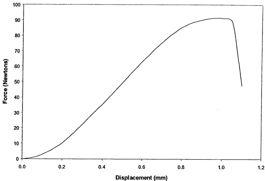
Figure 3. Force-displacement curve EPON 828/EPI-CURE 3290 polymer thin film.
