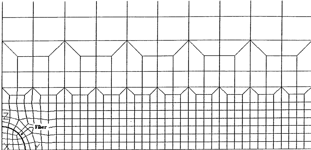
Figure 22. Finite element analysis mesh for \frac{1}{4} fiber model.
