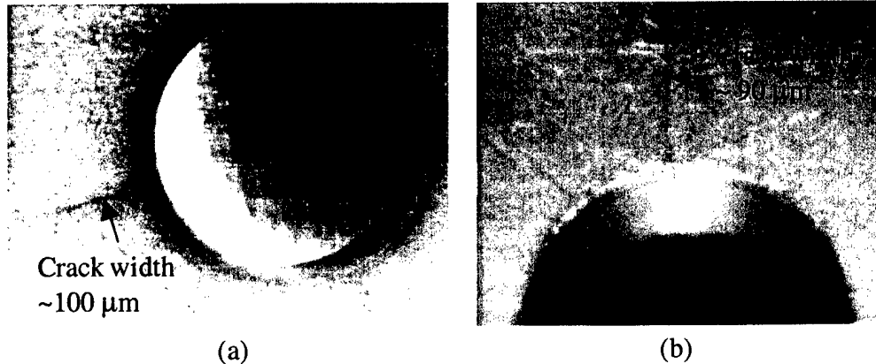
Fig.7 Mid-IR CCD images at 3\ \mu\text{m} - 5\ \mu\text{m} for (a) Sandia demo crack sample consisting of a rivet and a rivet-hole-induced crack underneath \sim 100\ \mu\text{m} -thick standard aircraft paint layer; and (b) a CCNY-LM crack sample consisting of a rivet-hole and rivet-hole-induced cracks covered by a typical military paint system #5 (strontium chromate epoxy low IR reflective primer covered by polyurethane topcoat paint) with a thickness of \sim 120\ \mu\text{m} .
