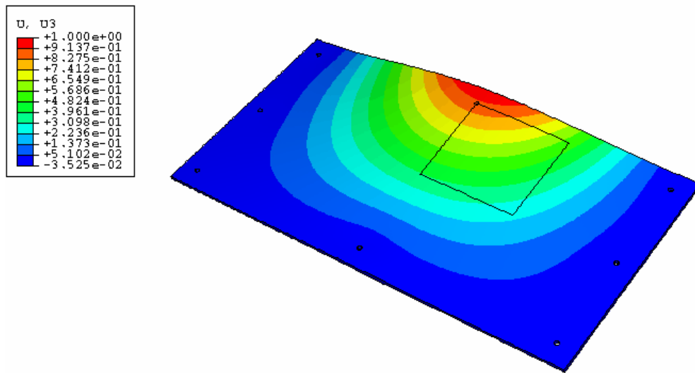
Figure 4.24. First Mode for Bolt 4 Removed 101.56 Hz Experimental
