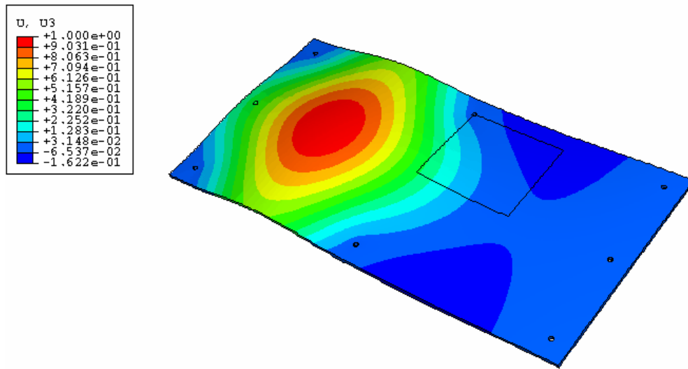
Figure 4.23. First Mode for Bolt 2 Removed 221.09 Hz Experimental
