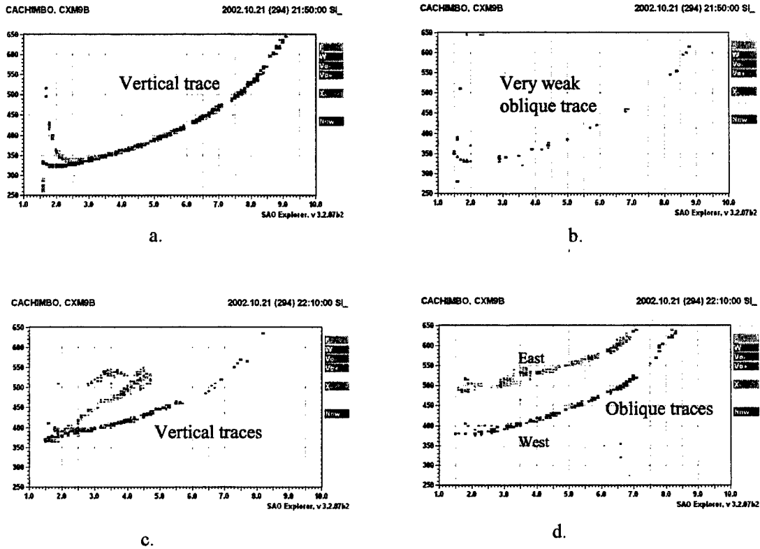
Figure 3. Cachimbo Ionograms 21 October 2002.
