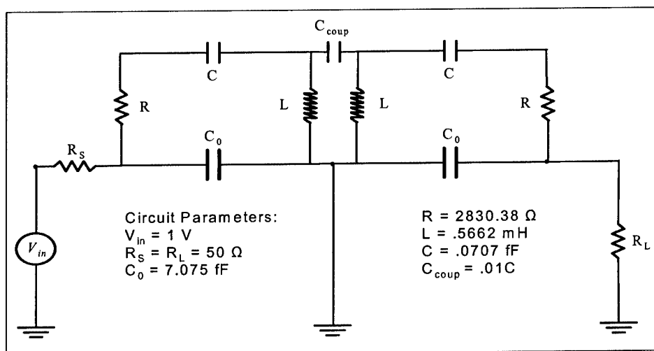
Figure 6.16: Equivalent circuit for coupled SCF configuration; coupling tether represented by coupling capacitor ( C_{coup} ).
