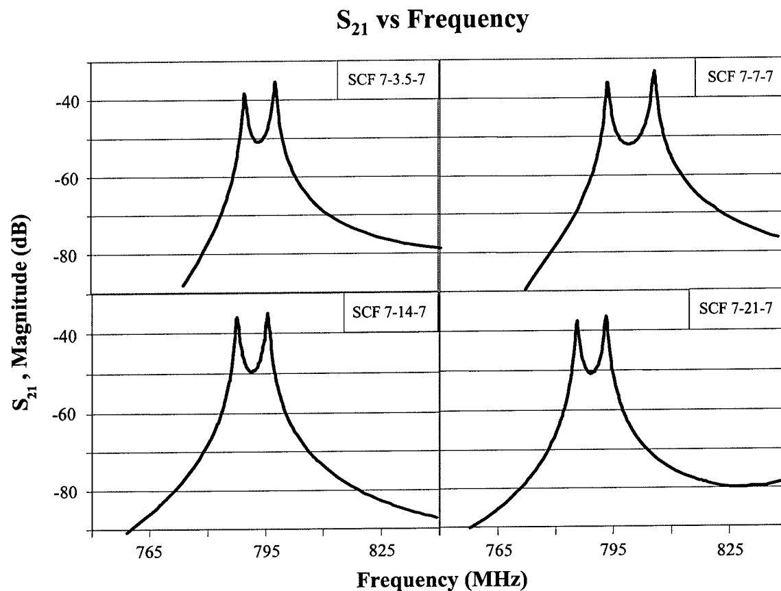
Figure 6.14: SCF transfer functions for various coupling tether lengths. The legend notation is the same as that used for Fig. 6.4.
