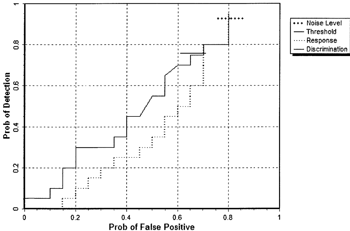
Figure 2. EM61 MKII blind grid probability of detection for response and discrimination stages versus their respective probability of false positive over all ordnance categories combined.
