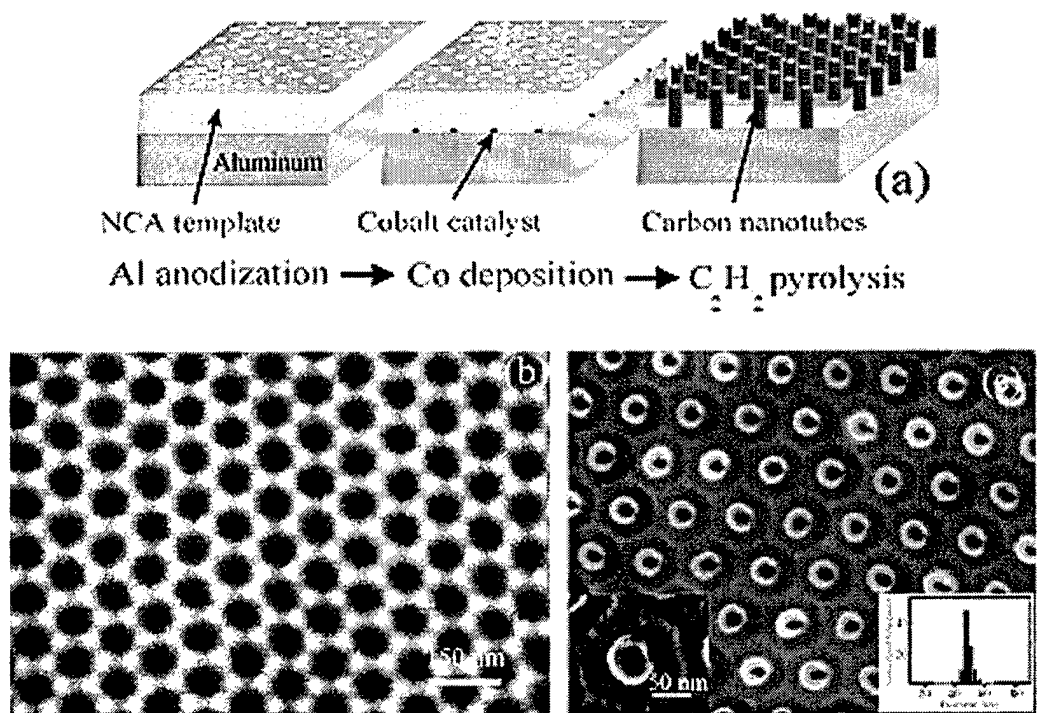
Figure 3. (a) Schematic of CNT array fabrication process. (b) NCA template after first anodization showing hexagonal texturing. (c) Highly-ordered CNT array formed using method in (a). Left inset is a close-up of the nanotube in its hexagonal cell. Right inset is a histogram of the nanotube diameter showing narrow size distribution around 47 nm.
