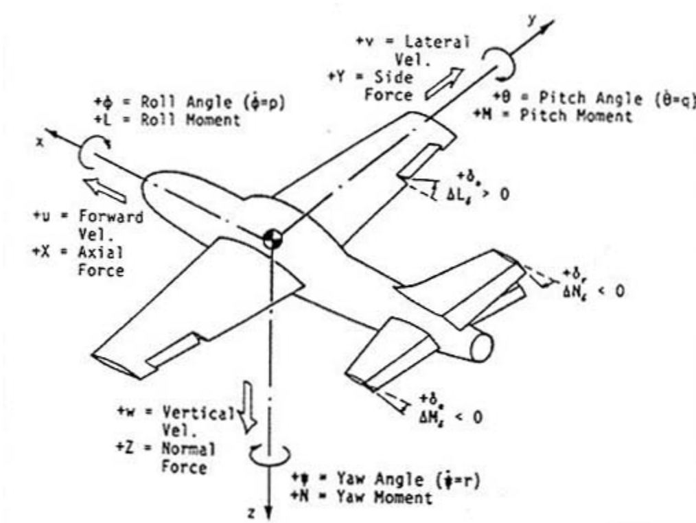
Figure 2. Illustration of Euler Angles (From: Ref. 4)
