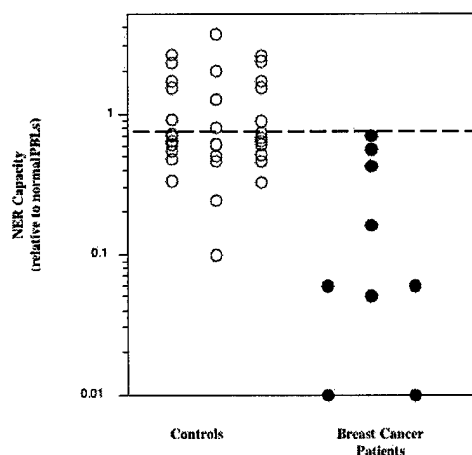
Figure 3. NER capacity of PBLs from disease-free controls ( N = 33 ) and newly diagnosed (pre-therapy) breast cancer patients. NER capacity was assessed with the UDS assay.
