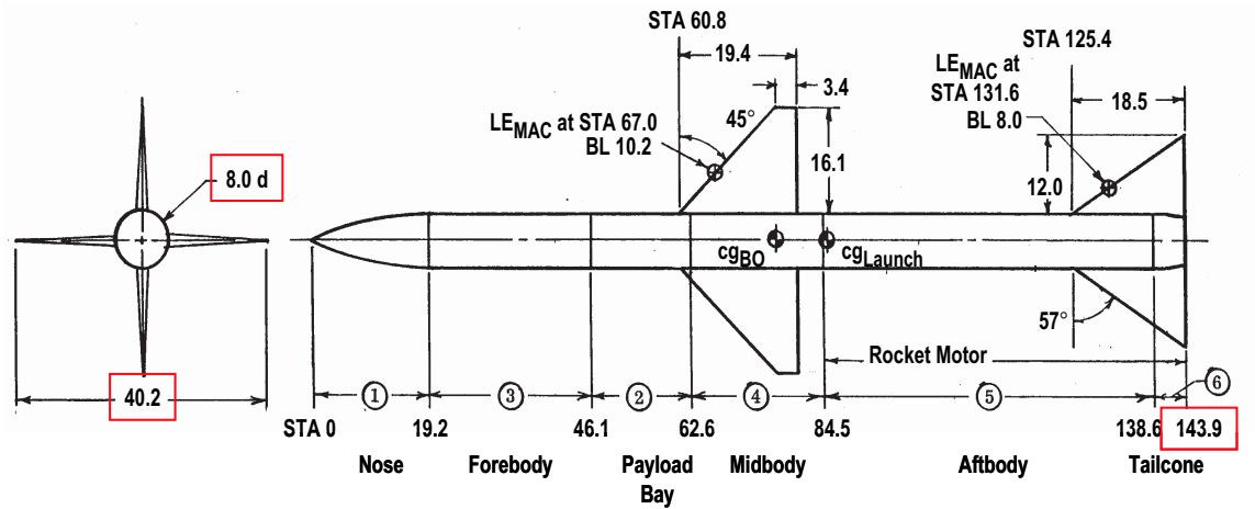
Figure 9: Baseline missile configuration
