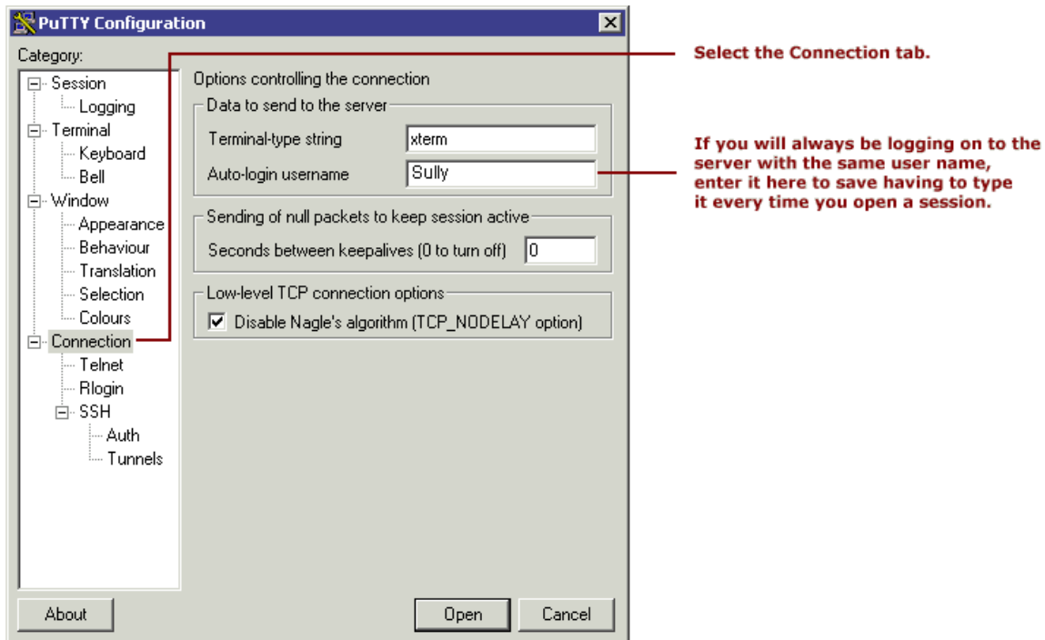
Figure 4.5. PuTTY Connections
