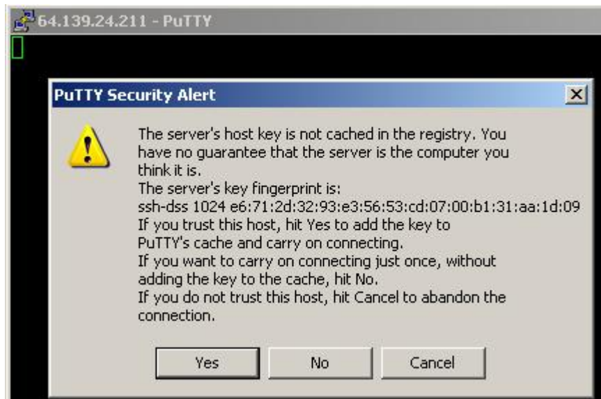
Figure 4.3. Initial SSH Connection Shows Server Fingerprint
