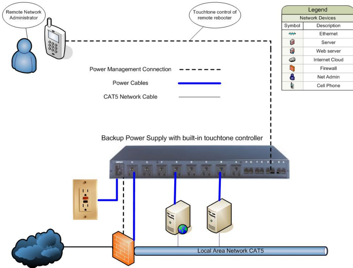
Figure 5.5. UPS with Remote Management via Built-in Touchtone Controller
