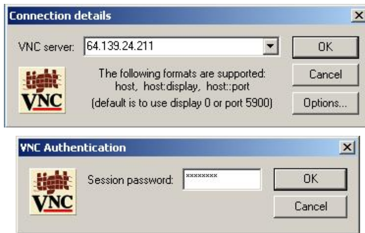
Figure 3.5. VNC Login Prompts
