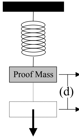
Figure 1. Gravimeter 2
