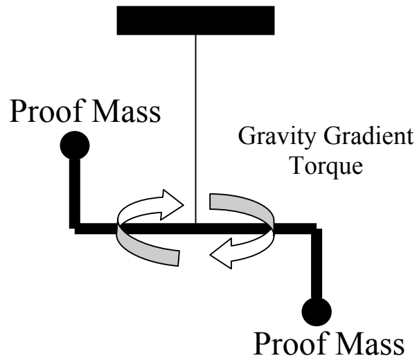
Figure 2. Torsion Balance 5
