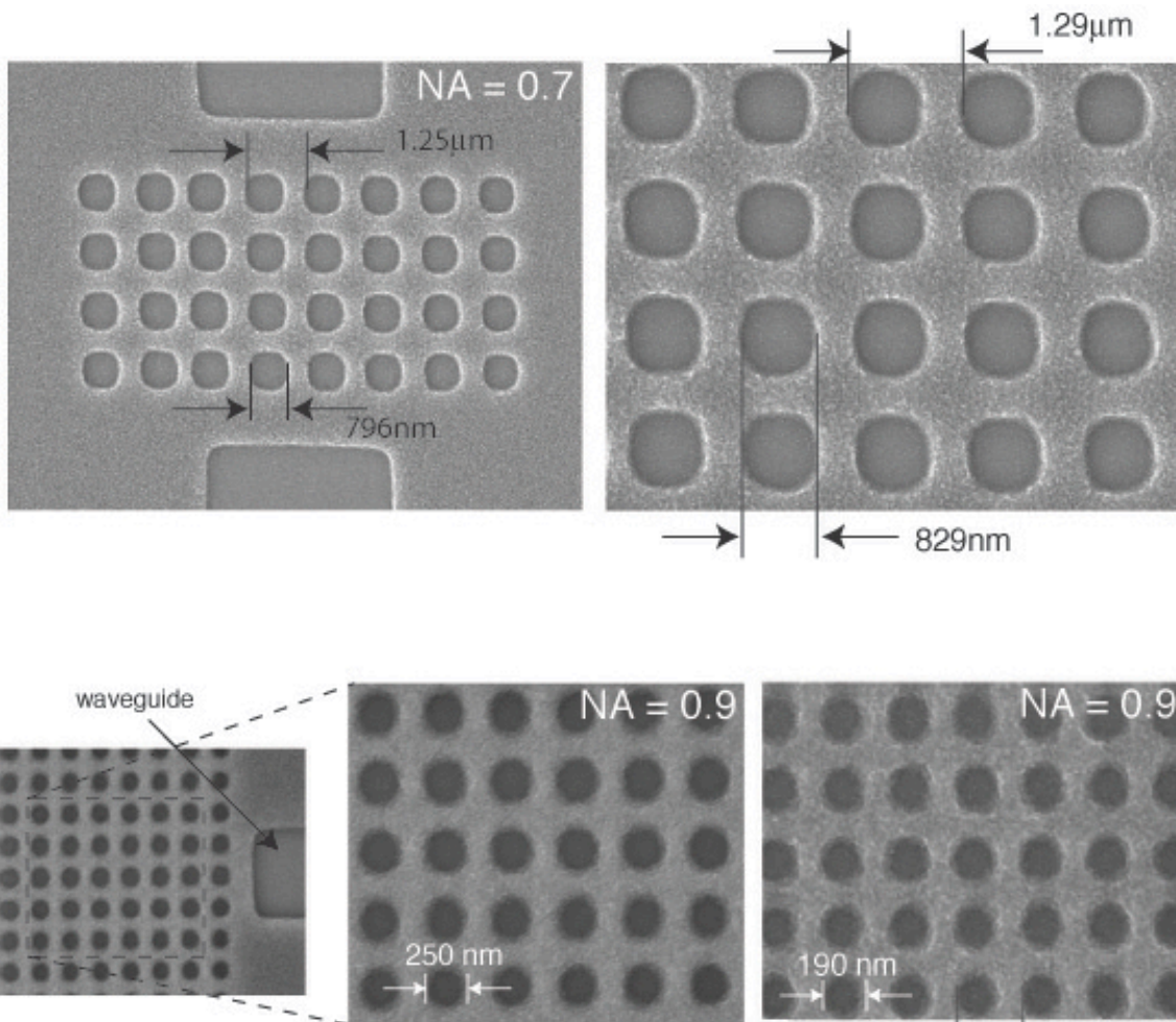
Figure 5 - 18. Scanning-electron micrographs of patterns exposed with the continuous-scan UV-ZPAL system. Top: 2D photonic bandgap structures with 1.29 \mu\text{m} period, Bottom: 2D photonic bandgap structures with 500 nm period, and also with 400nm period.
