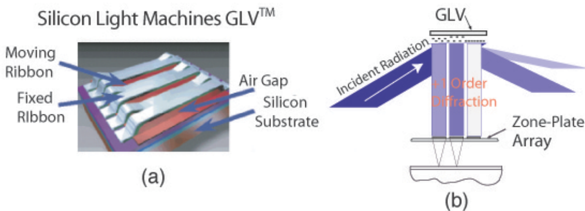
Figure 2 - 5. The Silicon Light Machines Grating Light Valve™ (GLV™) (a) one pixel of the GLV™ (each pixel can be thought of as a “mini-grating”), (b) intended implementation of the GLV™ with our linear array of zone plates indicating gray scaling.
