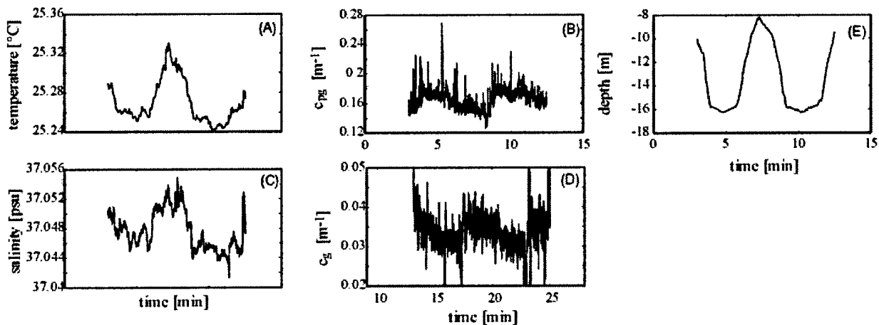
Figure 1. Transect.
