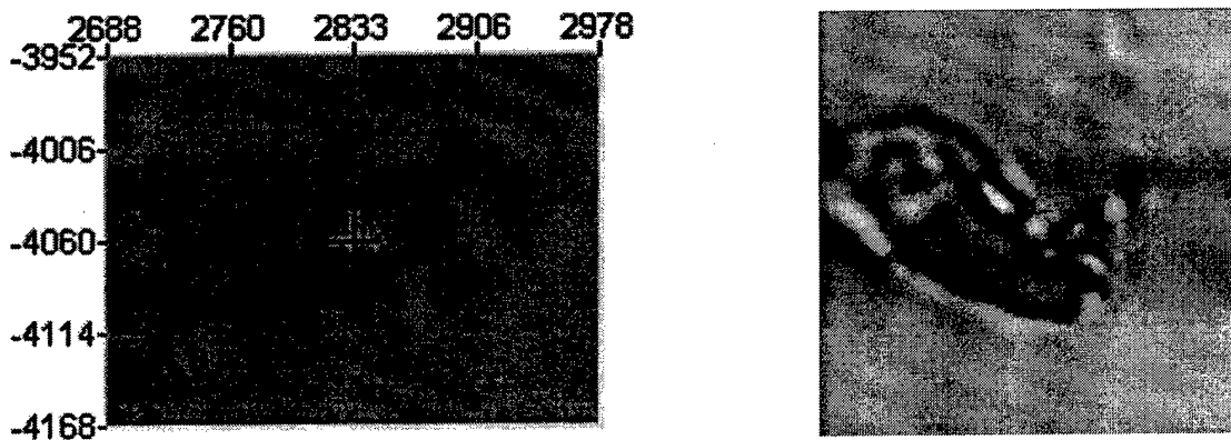
Figure 1: Comparison of optical image (left) and scanning near-field infrared (SNIM) image at \lambda = 10.6 \mu\text{m} of hair cross-section; near-field IR calibration standard (right) showing sub-wavelength spatial resolution ( 2 \mu\text{m} ).
