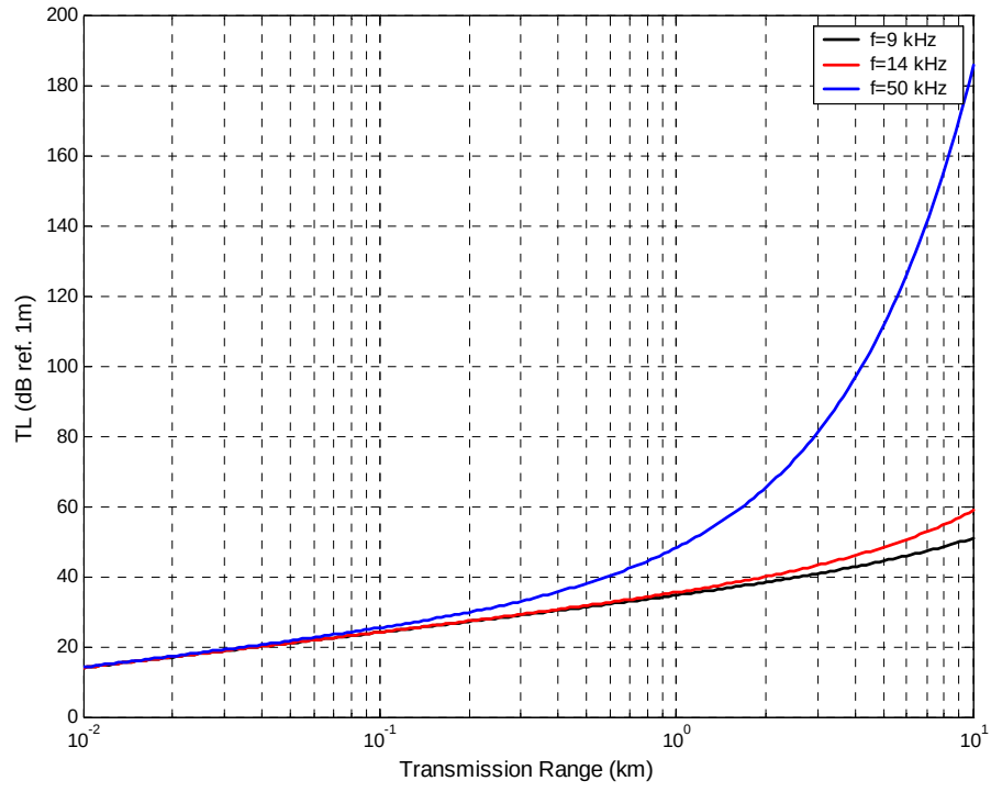
Figure 3. Range and Frequency Dependency of TL ( H=150\text{ m} , \theta_c=30^\circ ).
