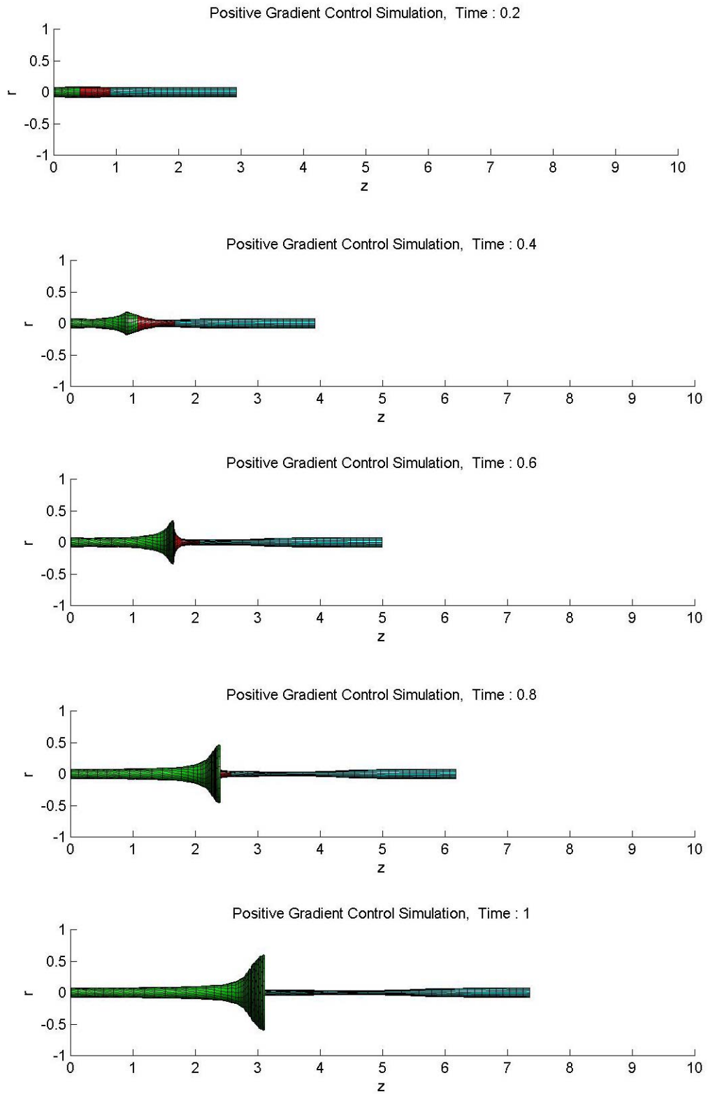
Figure 7-7: Positive gradient control simulation results, r=0.08
