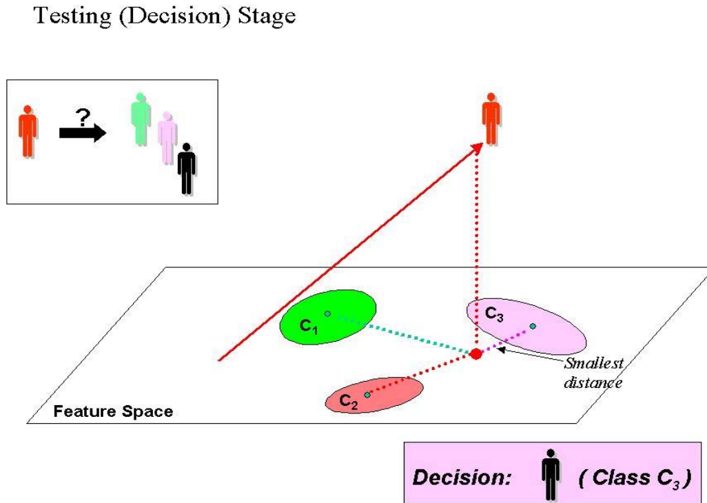
Figure 4. Testing Stage of Face Recognition (From Ref. 9.).
