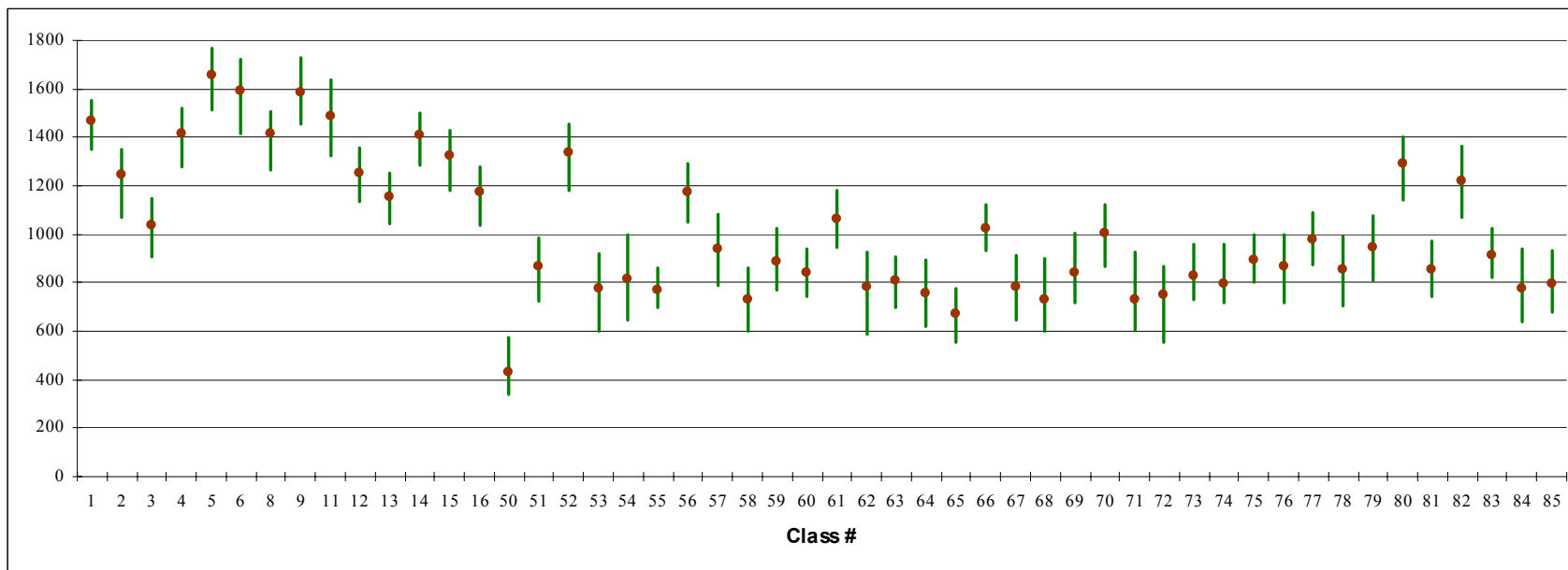
Figure 54. LDA-Based Classification.
